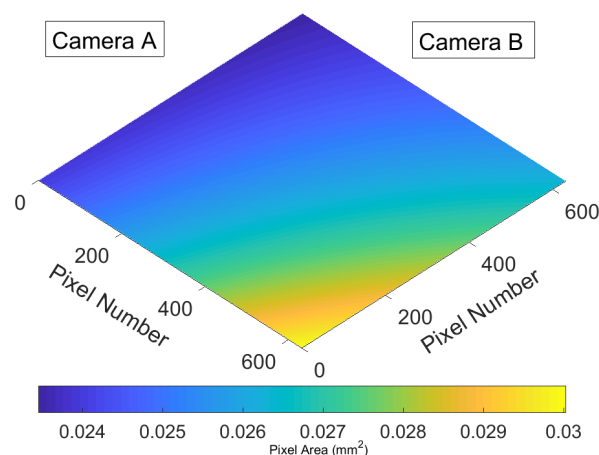
Figure 3. The effective area (in \text{mm}^2 ) of each pixel within the field of view for 2DVD SN074, as determined by using the measurements presented in Table 1. The geometry is shown to coincide with the orientation presented in Figure 2.
