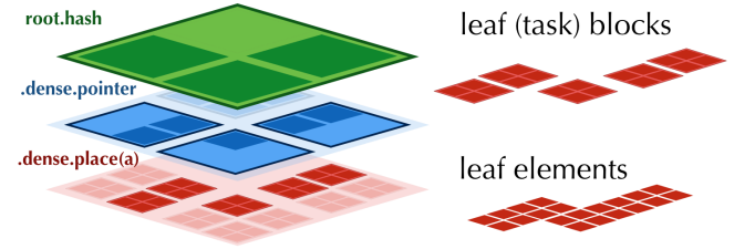
Fig. 5. In our language, programmers define data structures by nesting elementary components such as hash tables and dense arrays. Kernels are defined as iterations over leaf elements (i.e., voxels or pixels), independent of the internal data organization. Leaf blocks , immediate blocks of leaf elements, are the smallest quantum of storage and computation tasks.
