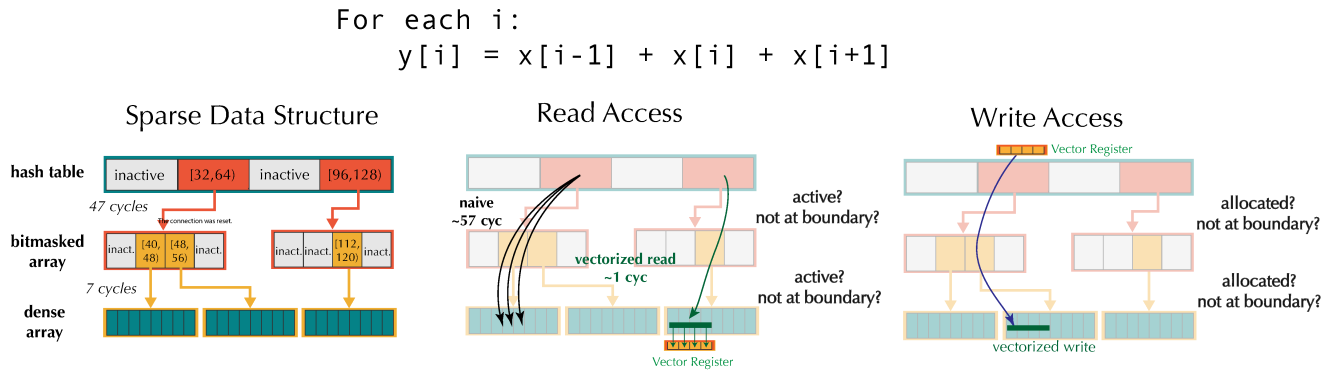
Fig. 2. Accessing a multi-level sparse array is significantly more involved than accessing a dense array. The figure illustrates an example three-level sparse array and the read and write access of a stencil y[i] = x[i-1] + x[i] + x[i+1] . Naive code is usually inefficient, since the hierarchy makes traversal costly, and it is especially problematic for spatially coherent accesses, where the top of the traversal is often redundant. Optimized and vectorized code needs to leverage access locality to amortize the access cost, check for sparsity, handle boundary cases, and allocate memory when necessary. Writing code for these accesses is tedious and error-prone, and it often leads to code that is highly-coupled with the data structure. Our language decouples the data structure implementation and the access, while our compiler automatically generates optimized code given the access pattern and the specific data structure. As a result, users write code as if they are accessing dense arrays, while having the freedom to change the data layout and sparsity representation without affecting the computation code.
