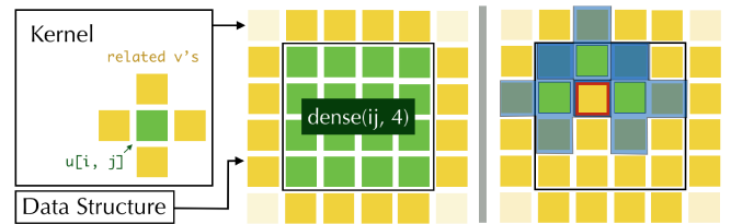
Fig. 7. Left and middle: Combining kernel and data structure information, the compiler will infer the elements required by this compute block. In this specific case, a 6 \times 6 scratchpad will be generated, covering region [-1, 5] \times [-1, 5] . Right: The v (yellow square with red border) element is loaded into shared memory, and then reused by u five times (three shown in green blocks with their stencil shown in semitransparent blue). By doing this we reduce data load-to-use latency and main memory bandwidth consumption significantly.
