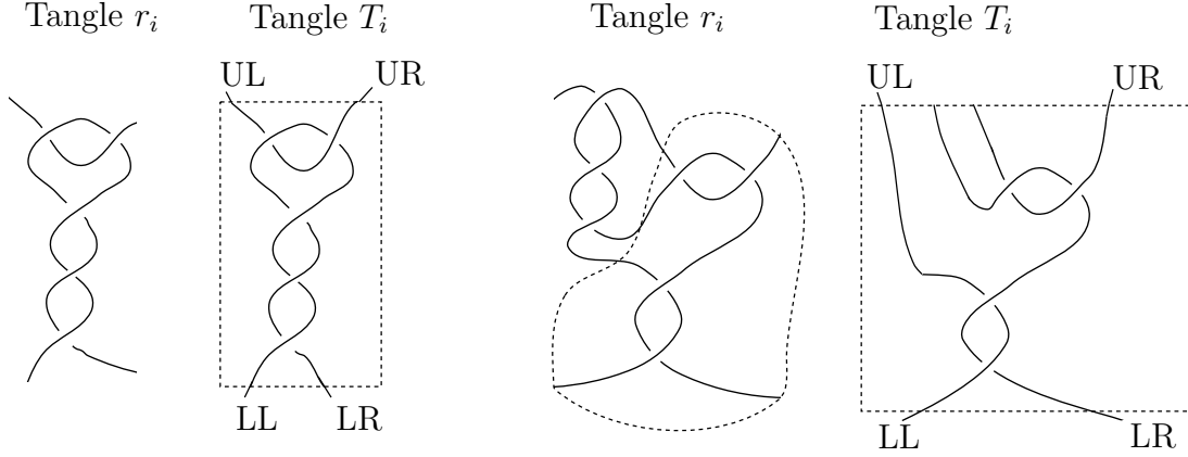
FIGURE 26. Two cases of the T_i 's corresponding to the r_i 's are shown. UL stands for upper left; UR stands for upper right; LL stands for lower left; LR stands for lower right.
