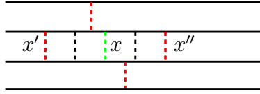
FIGURE 21. The crossing x corresponds to the green edge.
