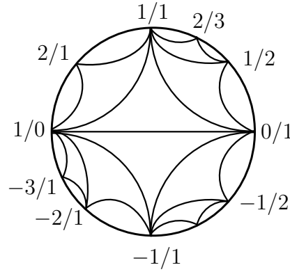
FIGURE 30. Some edges of the 1-complex \mathcal{D} .
