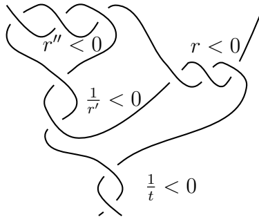
FIGURE 23. Any rational tangle is produced by a combination of TR-moves. In the picture shown, we have performed three TR-moves: first on 1/t , then r , then 1/r' .
