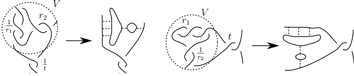
FIGURE 28. Examples of applying the all-$B$ state to $V$ and the resulting disjoint circles for moves sending tangles $\frac{1}{t}$ to $(\frac{1}{r_1} \oplus r_2) * \frac{1}{t}$ and sending $t$ to $(r_1 * \frac{1}{r_2}) \oplus t$. The tangles that form part of $V$ are encircled.
