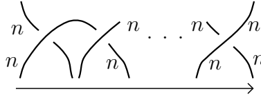
FIGURE 16. The arrow indicates the direction from left to right of the crossings in \mathcal{S}^t .
