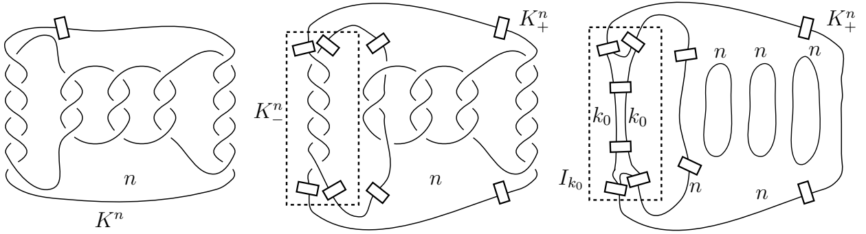
FIGURE 10. From left to right: K^n , doubling the idempotents and the splitting K^n = N(K_-^n \oplus K_+^n) , and N(I_{k_0} \oplus (K_+^n)_{\sigma_A}) , where \sigma_A is the Kauffman state that chooses the A -resolution on all the crossings in K_+^n . The dotted boxes enclose the skein elements in \mathcal{S}(D^2, 2n, 2n) , which are sums of 2n -tangles.
