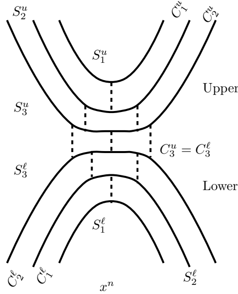
FIGURE 15. Local labeling of n^2 crossings on the all- B state of an n -cabled crossing. In this example n = 3 .
