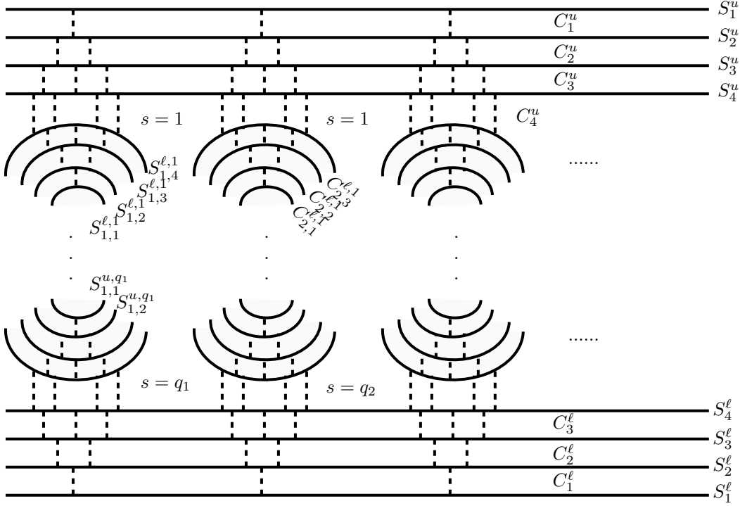
FIGURE 14. Labeling of crossings, arcs, and circles from applying the all- B state to K_+^n . In this example n = 4 .
