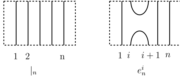
FIGURE 5. An example of the identity element |_n (left) and a generator e_n^i (right) of \text{TL}_n for n = 5 and i = 2 .
