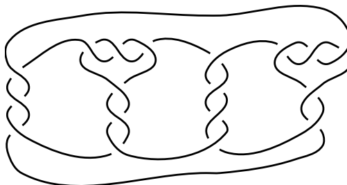
FIGURE 2. The Montesinos link K(-\frac{1}{3}, -\frac{3}{10}, \frac{1}{4}, \frac{3}{7}) .
