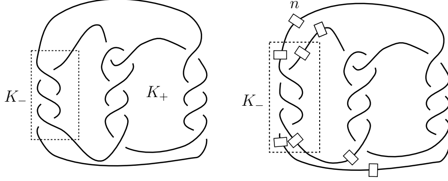
FIGURE 24. A special Montesinos knot K = K(-\frac{1}{3} = \frac{1}{-2+\frac{1}{-1}}, \frac{2}{7} = \frac{1}{3+\frac{1}{2}}, \frac{1}{4} = \frac{1}{3+\frac{1}{1}}) = N(K_- \oplus K_+) , and K^n = N(K_-^n \oplus K_+^n) .
