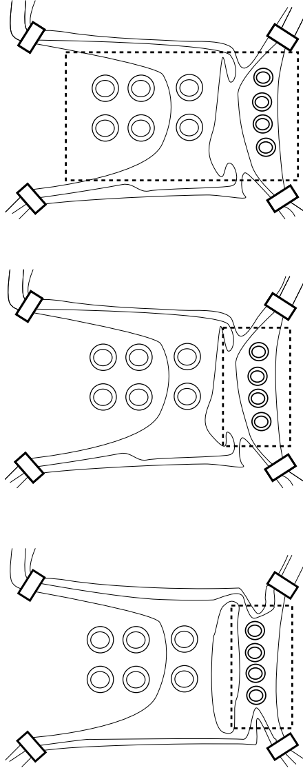
FIGURE 11. Top: an example of (K_+^n)_\sigma with n = 3 and c(\sigma) = 4 . Middle: when restricting \sigma to i = 4 th twist region, we have c_4(\sigma) = k_4(\sigma) = 2 . Bottom: we show an example of a state \sigma where c_4(\sigma) = 1 and therefore k_4(\sigma) = \lceil \frac{1}{2} \rceil = 1 .
