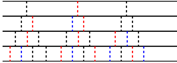
FIGURE 19. An example of F_\tau with edges shown in blue with the minimal state \tau shown as red edges.
