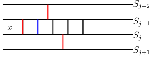
FIGURE 18. Only the blue edge is in R_x because of the presence of the top and bottom red edges.
