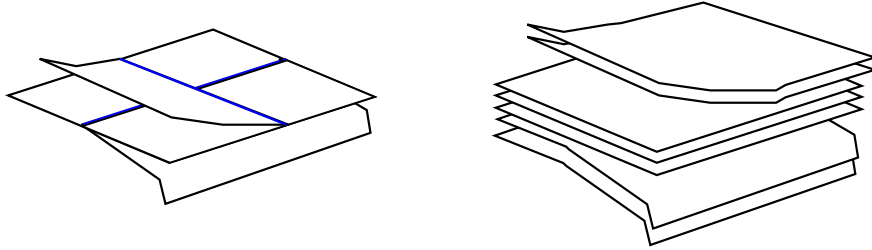
FIGURE 29. Left: local picture of a branched surface, with the blue lines indicating the singularities. Right: a surface carried by the branch surface.
