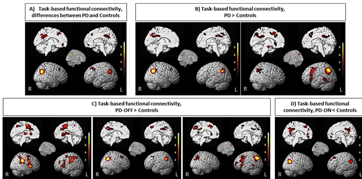
Fig. 3 – The results of meta-analytic connectivity modeling analysis in BrainMap data set. Task-based connectivity pattern of the seed based on ALE findings. All activations are significant at p < .05 corrected for multiple comparisons using the family-wise error rate in cluster level (cFWE).
