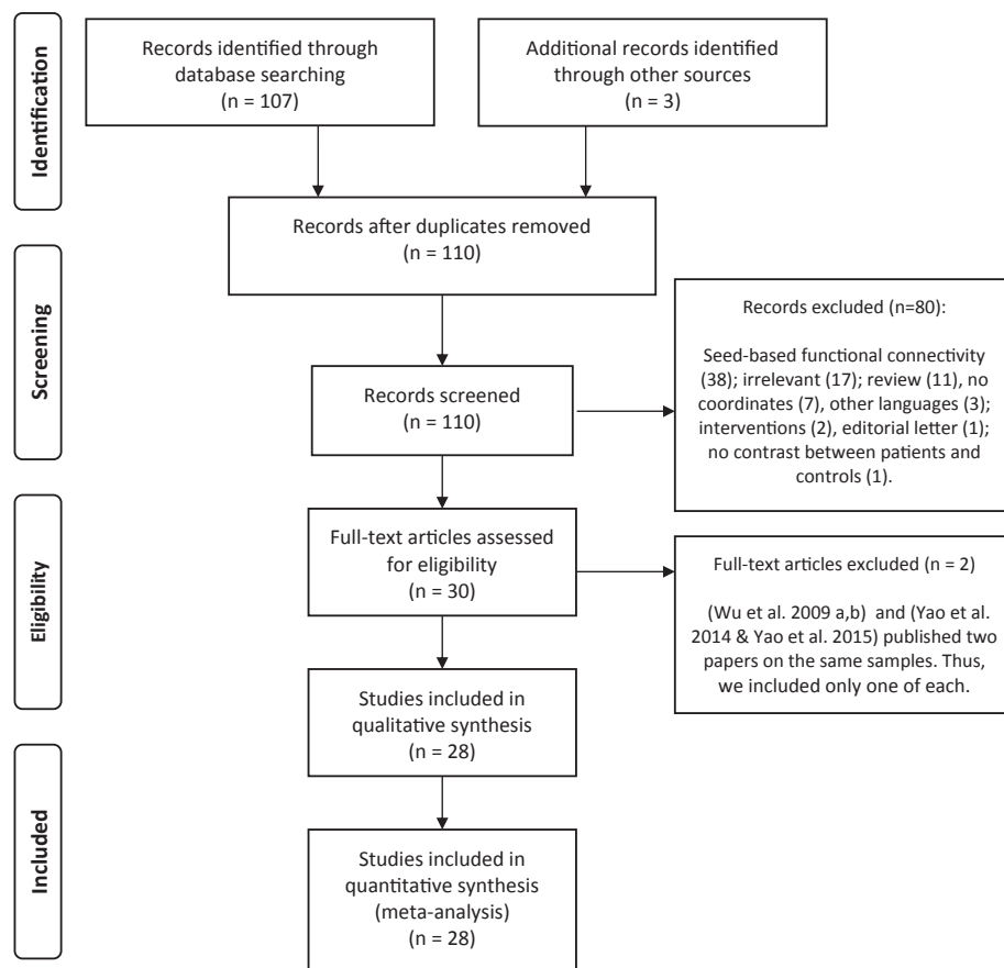
Fig. 1 – Paper selection strategy flow chart.
