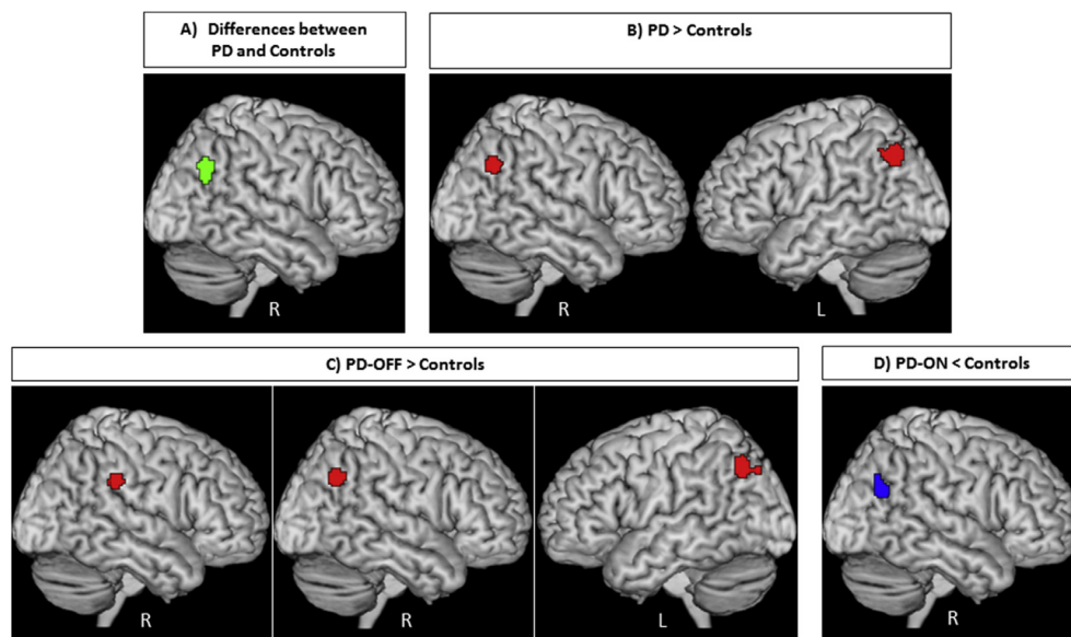
Fig. 2 – A) Convergence of aberrant (green) and B) convergence of increased (red) resting-state fMRI findings in patients with Parkinson's disease compared to healthy controls in bilateral parietal lobule. C) Convergence of increased (red) resting-state fMRI findings in patients with Parkinson's disease in the OFF-state compared to healthy controls in the right supramarginal gyrus and bilateral parietal lobule; D) Convergence of reduced (blue) resting-state fMRI findings in patients with Parkinson's disease in the ON-state compared to healthy controls in the right parietal lobule. All activations are significant at p < .05 corrected for multiple comparisons using the family-wise error rate in cluster level (cFWE).
