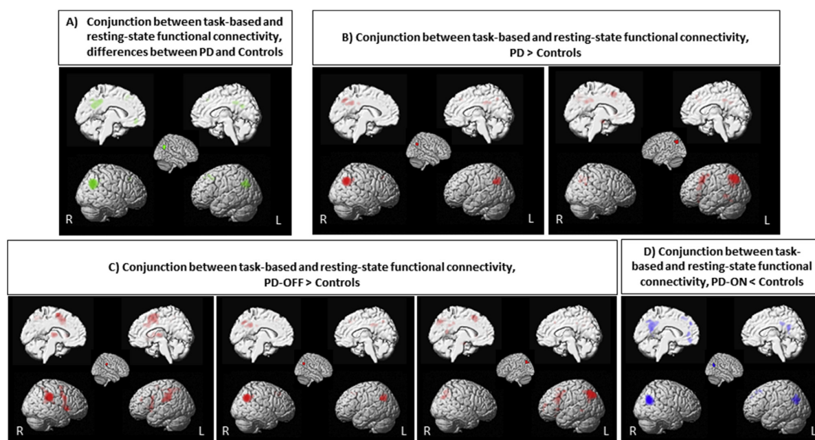
Fig. 5 – Conjunction analysis demonstrated regions significantly co-activated with seeds in task-based and task-independent data sets.
