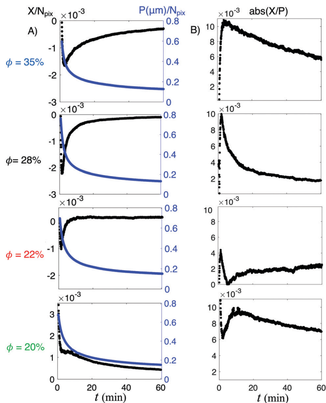
Fig. 5 Effect of particle density on the Minkowski measurements at B = 7.5 Gauss. (A) The Euler characteristic and boundary length as a function of time. (B) The absolute value of Euler over boundary length; which represents the curvature in 2D. Note how the “curvature” decreases over time to reach a more energetically favorable boundary, but in the case of \phi = 22\% , the system goes through a curvature of zero after approximately 5 min, implying that the system passes through a spinodal structure that coarsens and then breaks up into clusters.
