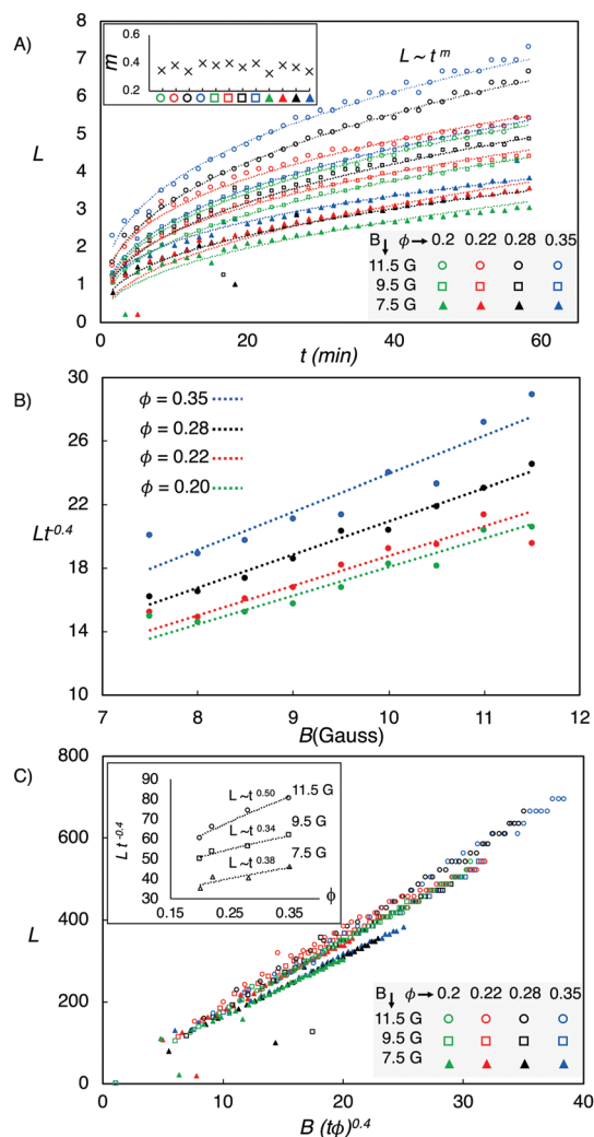
Fig. 6 Length scale correlation with system parameters: time, field, and concentration. (A) Power law relation between length scale and time, which corresponds to L \sim t^{0.4} . Inset shows the value of m for each data set. (B) Linear proportionality between the scaled length scale and magnetic field. (C) Master plot that incorporates all conditions that will help predict L as a function of t at any B and \phi . Inset shows the power law dependence on concentration.
