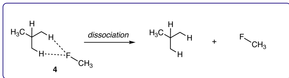
Scheme 3. Dipolar interaction of a C–F bond with proximate methyl groups.
