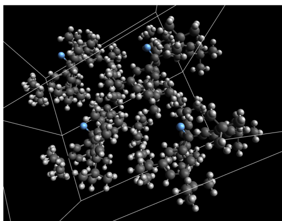
Scheme 2. Packing diagram of the crystal of 2 .
