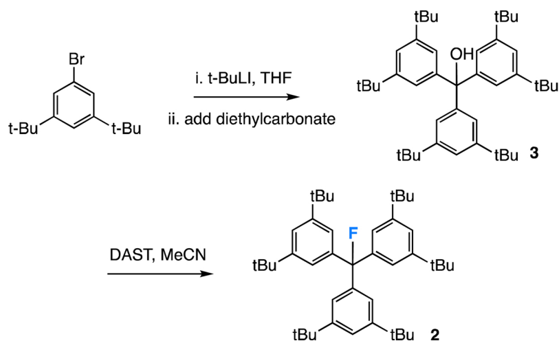
Scheme 1. Synthesis of 2 .
