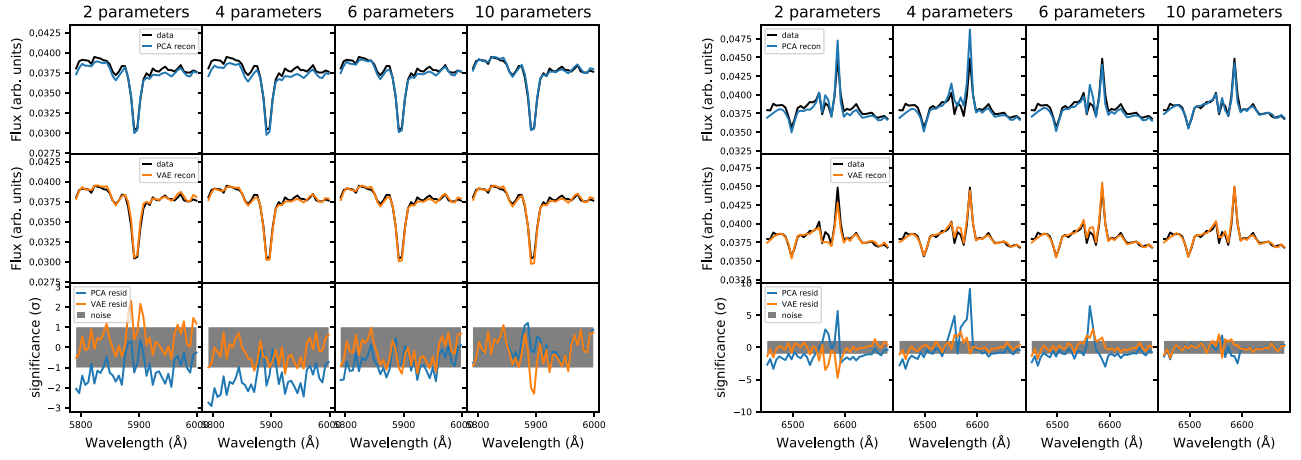
Figure 4. High-S/N quiescent galaxy (Plate-MJD-Fiber 394-51913-561): principal component analysis (PCA) and VAE reconstructions of the Na 5896 absorption line (left) and N II 6585/6588 and H \alpha emission lines (right). The noise band represents the SDSS stated pixel uncertainties. The median S/N of the spectrum is 78 in the left panel and 102 in the right panel. Both reconstructions find the significant Na absorption and N II emission with only two components, but the VAE provides a better reconstruction overall than PCA with the same number of components.
