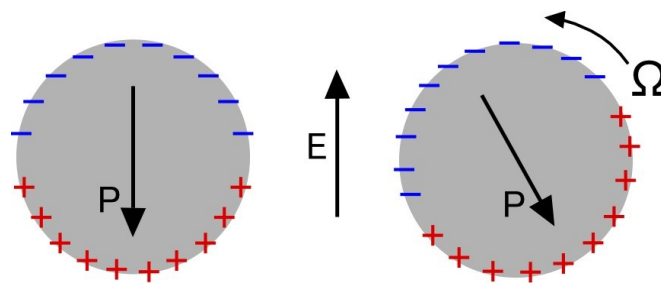
Fig. 1 (left) Induced free charge distribution for a sphere with R/S < 1 . (right) Above a critical field strength E > E_Q steady rotation in the plane perpendicular to the electric field ( \Omega \cdot E = 0 ) is induced by the misaligned induced dipole of the particle.
