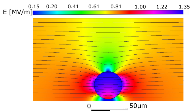
Fig. 9 Electric field magnitude (color) and potential lines about a sphere with d = 40 \mu\text{m} between two parallel electrodes separated by a 120 \mu\text{m} gap. Particle conductivity is \sigma_p = 10^{-17} \text{ S/m} and the medium conductivity is \sigma_m = 2 \times 10^{-8} \text{ S/m} . The potential difference is 90V and the particle is suspended at a height of 2.8 \mu\text{m} above the bottom electrode. Computations performed with ANSYS-FLUENT.
