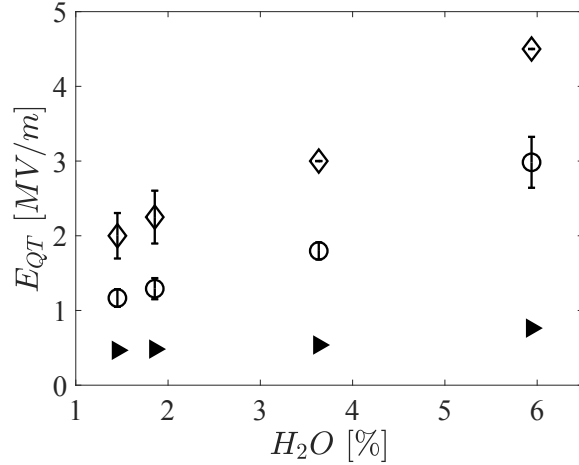
Fig. 6 Quincke rolling thresholds for 0.1 M AOT-hexadecane solution as a function of moisture content. The symbols correspond to particle confinement \diamond : d/h = 0.83 , and \circ : d/h = 0.17 . The solid symbols are the threshold for unconfined electrorotation calculated from Eq.(1) using the conductivities corresponding to the 0.1M AOT and moisture content, Table 2.
