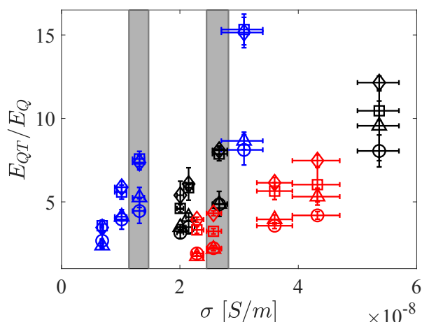
Fig. 7 Quincke rolling threshold as a function of conductivity of the suspending fluid. The symbols correspond to different confinement \diamond : d/h = 0.83 , \square : d/h = 0.42 , \triangle : d/h = 0.33 , \circ : d/h = 0.17 . Colors denote AOT concentration 0.05 M (blue), 0.1 M (black) and 0.15 M (red). The electric field is scaled by the Quincke threshold for unconfined rotation calculated from Eq.(1) for the conductivity of the moisture-free fluid. The regions shaded in grey show that even for solutions with similar conductivities and same confinement, the E_{QT} can vary due to different moisture content.
