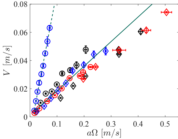
Fig. 5 Roller speed V versus the no-slip rolling velocity a\Omega , V = f(\delta)a\Omega , for the lowest ( \circ ) and highest ( \diamond ) moisture contents at 0.05 M (blue), 0.1 M (black), and 0.15 M (red) AOT and d/h = 0.83 . The dashed line corresponds to the case of rolling with no slip f(\delta) = 1 . The solid line is the velocity corresponding to a \delta = 10\text{nm} gap between the sphere and the bottom surface, calculated from Eq.(6).
