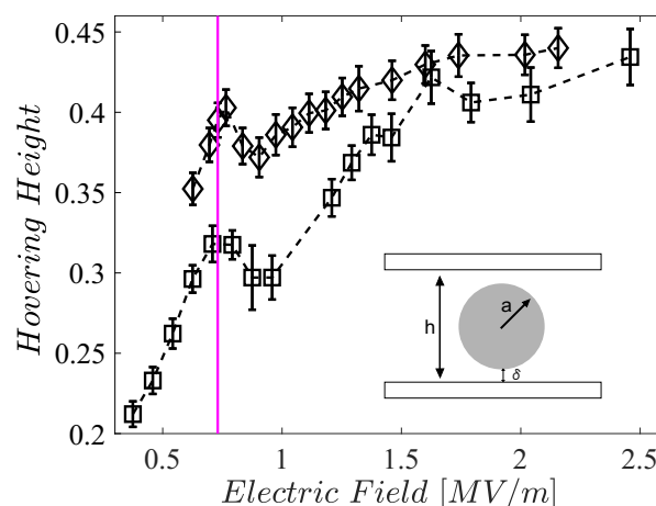
Fig. 10 Hovering height scaled by the distance between the electrodes, (a + \delta)/h , as a function of electric field for a 0.15M dry AOT and confinement d/h = 0.83 and d/h = 0.42 . The onset of rotation is marked by the magenta line. Hovering height of 0.5 corresponds to the midplane between the electrodes.
