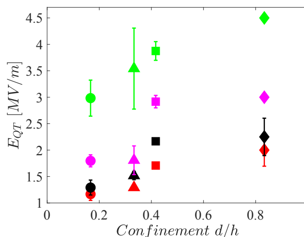
Fig. 4 Quincke rolling thresholds E_{QT} at different confinement for 0.1 M AOT in hexadecane and varying moisture content \%wt_{H_2O} = red < black < magenta < green (see Table 2 for the values of the water weight percentages). For comparison E_Q for this system is 0.37 MV/m in the absence of moisture.
