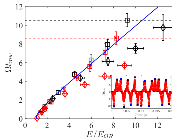
Fig. 12 Rotation rate of the hovering Quincke rotor for 0.1 M (black) and 0.15 M (red) AOT. The confinements are \diamond : d/h = 0.83 , and \square : d/h = 0.42 . The solid line is obtained from Eq.(3) using the experimentally determined E_{QR} instead of E_Q . The onset of the chaotic regime is marked by the black and red horizontal lines for 0.1 M and 0.15M respectively. The inset illustrates the chaos in rotation.
