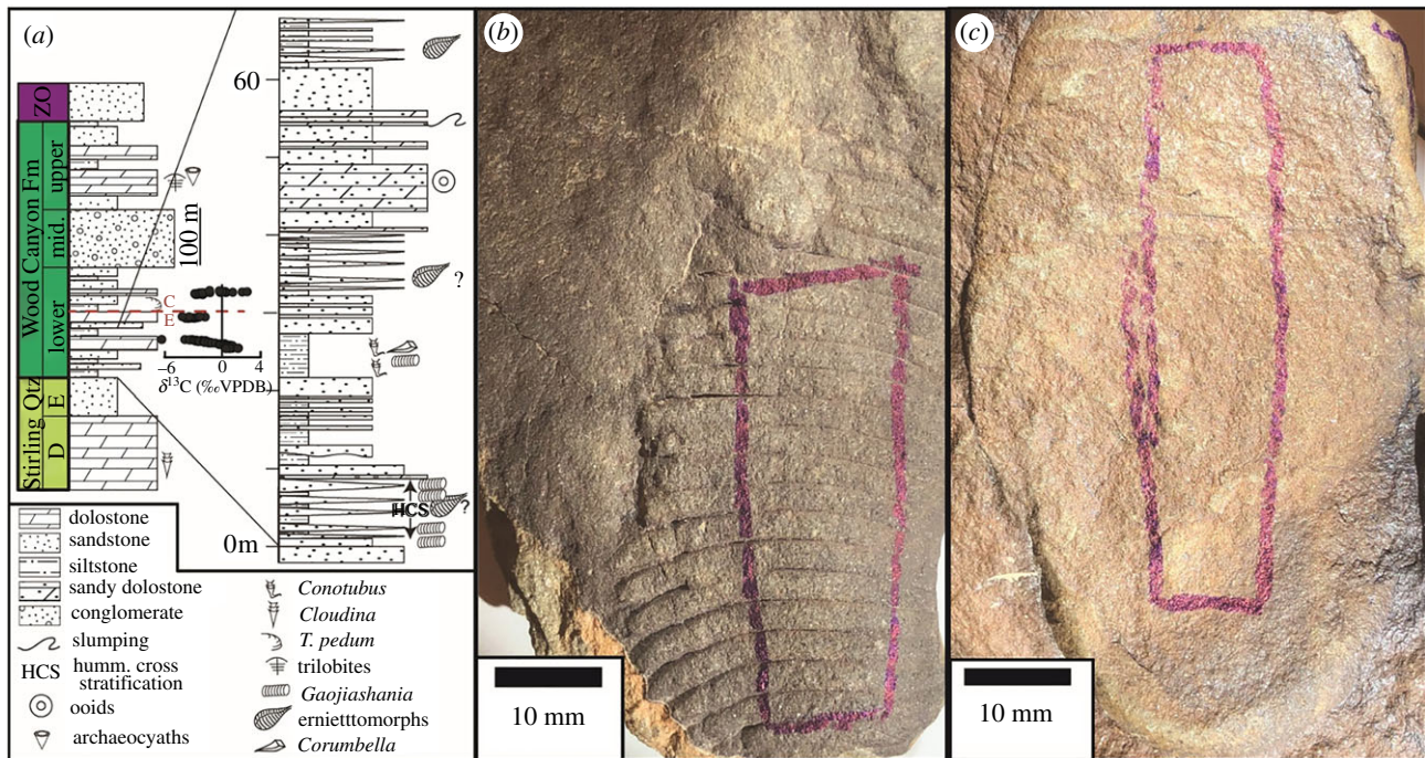
Figure 1. (a) Stratigraphic section of the Montgomery Mountains, Nevada area from Smith et al. [39]. (b) Ernettomorph fossil with mm-scale ridges. (c) Ridgeless erniettomorph fossil. The boxed regions show the lines along which the fossils were cut for thin sectioning and analyses.
