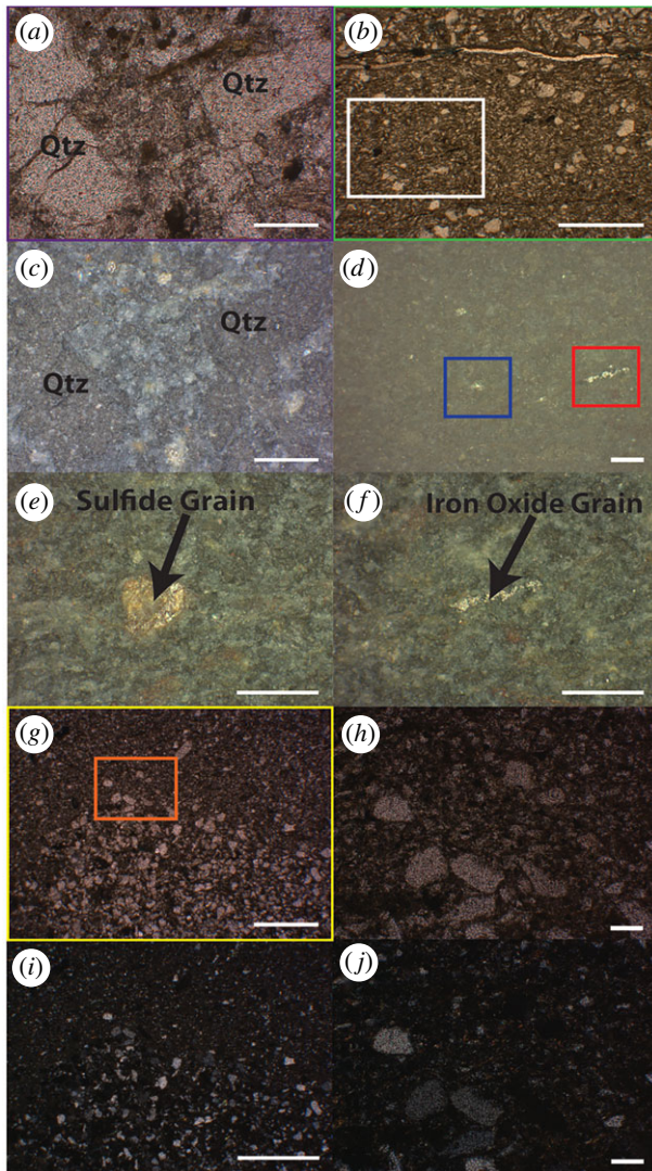
Figure 4. Photomicrographs of the ridged fossil ( a–f ) and the ridgeless fossil ( g–j ). Plane-polarized transmitted light ( a,b,g,h ), plane-polarized reflected light ( c–f ) and cross-polarized transmitted light images ( i–j ). The areas shown in ( a,b,g ) are identically coloured rectangles (purple, green, yellow) within the photomosaics in figure 3. ( e,f ) Sulfides and oxides in the blue and red boxes in ( d ), respectively, are sparsely distributed throughout the sample. ( i,j ) Clay minerals in cross-polarized transmitted light are more birefringent than surrounding quartz grains. Scale bar in ( b ) is 1 mm, all others are 100 \mu\text{m} .
