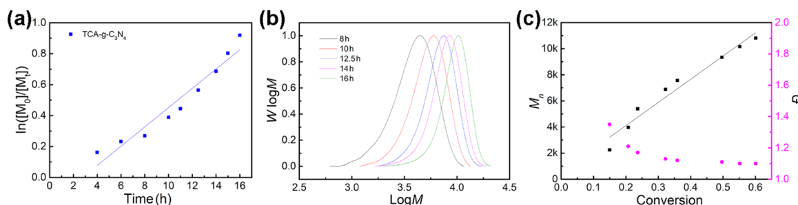
Figure 5. Kinetic study of TCA-g-C 3 N 4 -catalyzed PET-RAFT polymerization of MMA using CPADB as the CTA under blue LED irradiation ( \lambda_{\text{max}} = 465 nm, 3 mW/cm 2 ). The molar ratio of [MMA]/[CPADB] = 200:1 in 1 mL of DMSO: (a) \ln([M]_0/[M]_t) vs irradiation time and the fitted kinetic curve. (b) GPC profiles of poly(methyl methacrylate) (PMMA) synthesized in the kinetic study. (c) Number average molecular weight ( M_n ) and dispersity ( D ) of PMMA obtained in the kinetic study.
