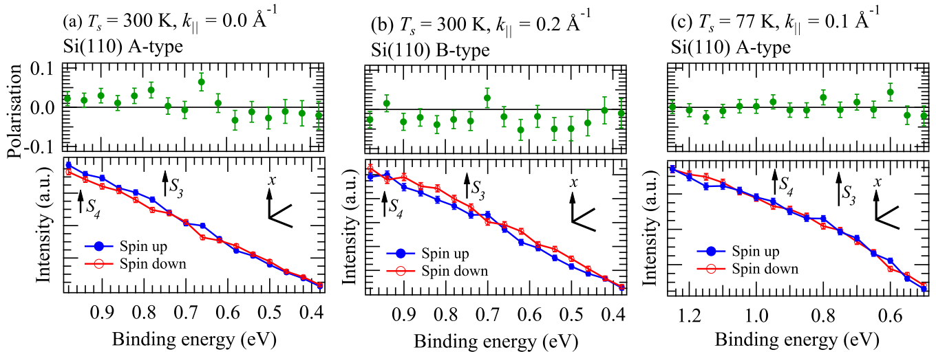
FIG. 11. (a) and (b) Longitudinal spin polarizations for an A-type and B-type Si(110)“16×2” surface at 300 K and k_{||} = 0.0 \text{ \AA}^{-1} and k_{||} = 0.2 \text{ \AA}^{-1} , respectively. (c) Longitudinal spin polarizations for an A-type Si(110)“16×2” surface at 77 K and k_{||} = 0.1 \text{ \AA}^{-1} . The corresponding spin-up (filled blue circles) and spin-down (empty red circles) intensities are shown in the lower panels. Polarizations shown in (a) and (b) were obtained with an energy resolution of 72 meV and those in (c) obtained with a resolution of 36 meV. Coordinate axes correspond to those shown in Fig. 3.
