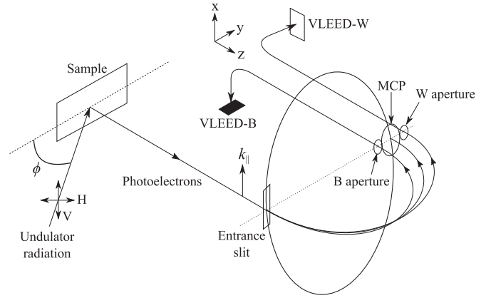
FIG. 3. Schematic diagram of the end station setup at the APE-LE beamline of the Elettra Sincrotrone Trieste. Undulator radiation was either horizontally (H) or vertically (V) polarized and incident at an angle of \phi = 45^\circ . The surface crystal momentum that is resolved due to the orientation of the entrance slit to the hemispherical analyzer is labeled k_{||} . The detected spin polarization directions are specified by the coordinate system used for the VLEED-W ( P_x, P_z ) and VLEED-B ( P_y, P_z ) polarimeters.
