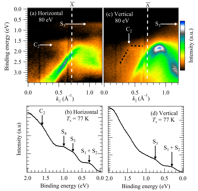
FIG. 7. 77 K band-dispersion maps of positive k_{||} obtained using 80 eV horizontally polarized light for (a) and 80 eV vertically polarized light for (c). These were produced from an A-type single-domain Si(110)“16×2” surface (LEED pattern shown in Fig. 6). EDCs (b) and (d) were obtained by integrating over the surface crystal momentum axis (both \pm k_{||} ). The black dashed line indicates the downward dispersion of C_2 .
