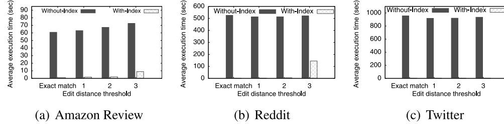
Fig. 28. Execution time of edit-distance selection queries on the three datasets.
