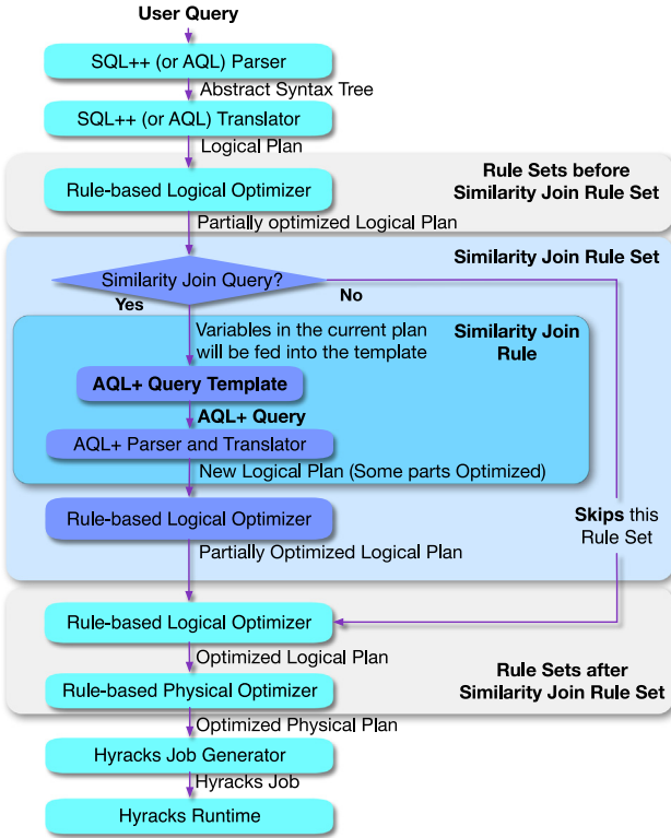
Fig. 20. Execution of a similarity-join query using AQL+.
