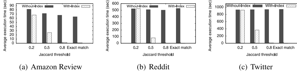
Fig. 27. Execution time of Jaccard selection queries on the three datasets.
