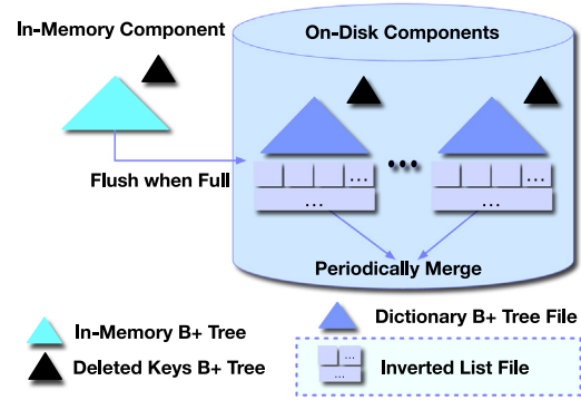
Fig. 7. The structure of an inverted index.
