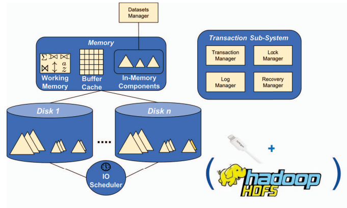
Figure 2. AsterixDB storage and memory management
