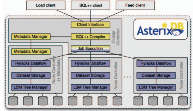
Figure 1. AsterixDB system schematic
