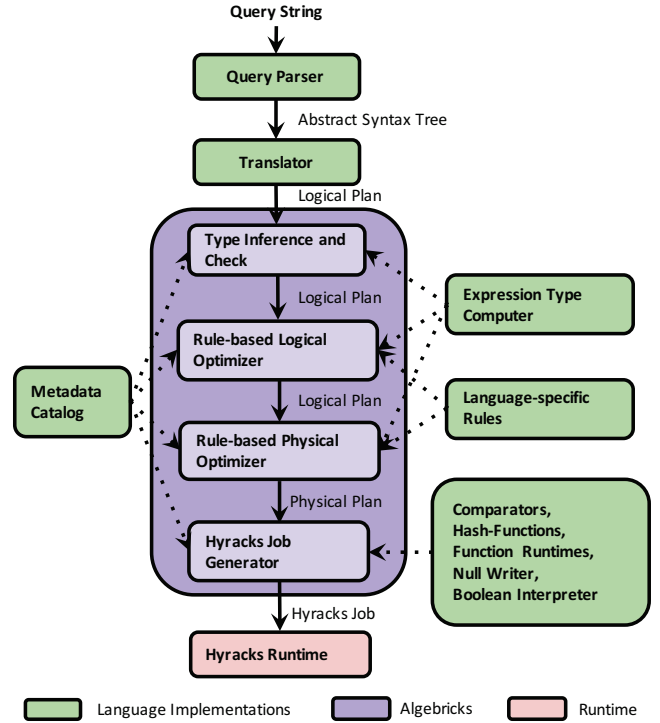
Figure 5. Algebricks query compiler framework
