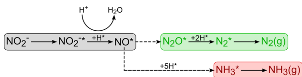
Scheme 1. Catalytic Reaction Pathways for \text{NO}_2^- Hydrogenation a
