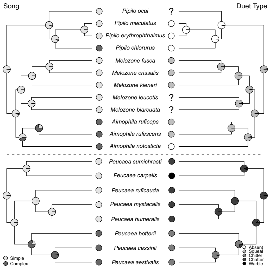
Figure 5 Trait reconstructions for song structure and duet type in two focal clades. Maximum-likelihood based trait reconstructions of song structure and duet type among the Peucaea and Aimophila clades with Character states are indicated by different shades of gray, and the probability of each character state is indicated by the proportion of that shade on the nodes.
