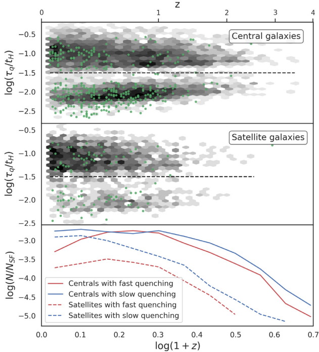
Figure 8. Final quenching times as a function of redshift, for z=0 quenched galaxies in SIMBA. Top: Hexbin plot of \log t_q/t_H of central galaxies versus \log(1+z_q) , with z_q the redshift at which the quenching ends. Green circles represent galaxies that experienced a rejuvenation prior to this final quenching. The horizontal black dashed line shows the demarcation between slow and fast quenching modes. Middle: Same as the top panel, but for satellite galaxies. Bottom: Fraction of star-forming galaxies that undergo quenching in each redshift bin, divided into centrals and satellites versus \log(1+z_q) .
