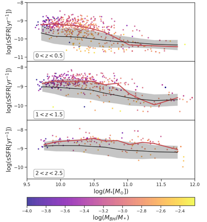
Figure 4. sSFR versus M_* in mergers identified via an increase of \geq 20 per cent in stellar mass relative to its progenitor at the previous snapshot (scatter points), within three redshift intervals (top to bottom panels). The merger points are colour coded with \log(M_{\text{BH}}/M_*) at the snapshot of the mass jump. The median of the population of galaxies not undergoing mergers is shown as the black solid line, with the grey shaded region representing the 1\sigma deviation in the data. The running median for the mergers is also shown in red. Galaxies that have just undergone a merger generally show elevated SFRs, but the ones with low sSFR tend to be ones with overmassive black holes.
