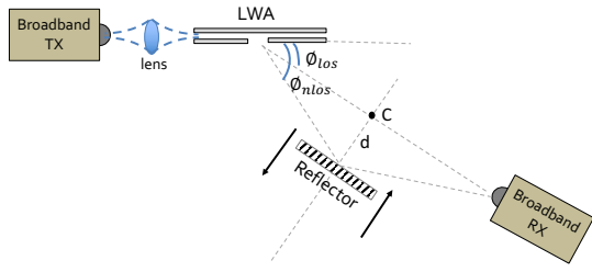
Figure 15: The schematic of our multipath experimental setup.
