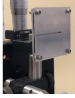
Figure 5: Our custom 4 \times 4 \text{ cm}^2 LWA.
