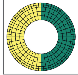
Figure 2: The mesh generated by the Python code shown in the main text. Cells are colored by material id.
