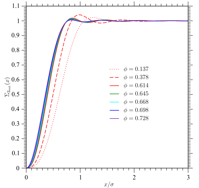
FIG. 11. The external part of the two-point correlation function \Sigma_{2\text{ext}}(x) at several values of packing fraction \phi representative of the equilibrium fluid (red: dotted, dashed, and continuous), metastable fluid (green), glassy (cyan and blue), and MRJ (indigo) states.
