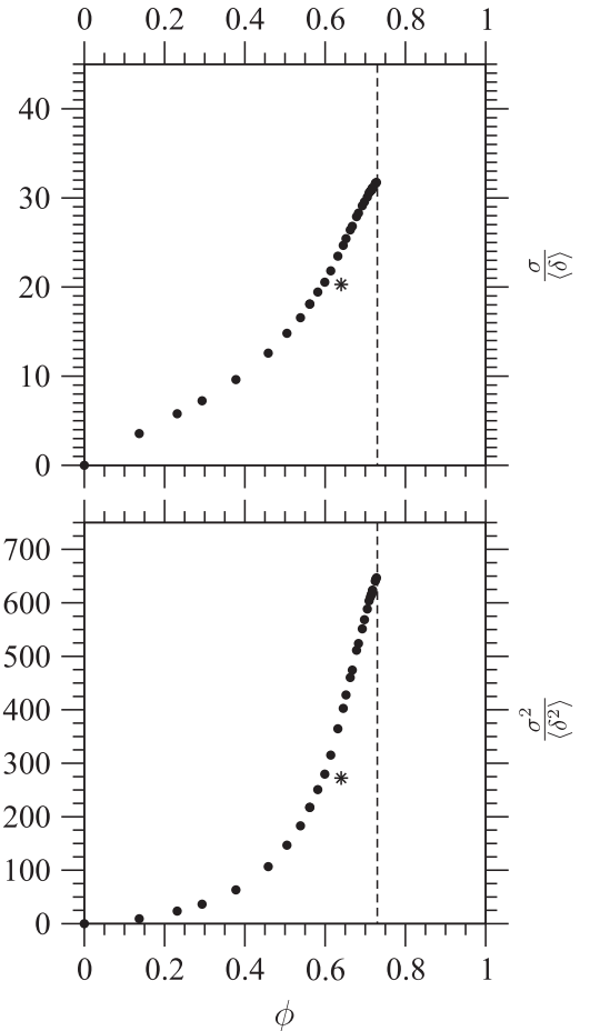
FIG. 14. Inverse of mean pore size \langle\delta\rangle and mean-square pore size \langle\delta^2\rangle as a function of packing fraction \phi . The vertical dashed lines mark the value of \phi of the optimal-lens MRJ state. The asterisks are the corresponding data for the hard-sphere MRJ state.
