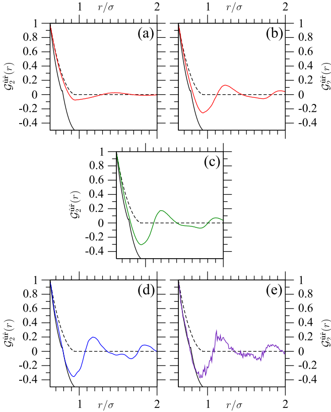
FIG. 7. Pair-correlation function G_2^{\text{ur}}(r) at several values of packing fraction \phi representative of the equilibrium fluid [(a) \phi = 0.378 ; (b) \phi = 0.614 ], metastable fluid [(c) \phi = 0.645 ], glassy [(d) \phi = 0.698 ], and MRJ [(e) \phi = 0.728 ] states. In each panel, the black curves correspond to the limit forms this function takes on when calculated considering two randomly chosen lenses either free (dashed) or touching (continuous).
