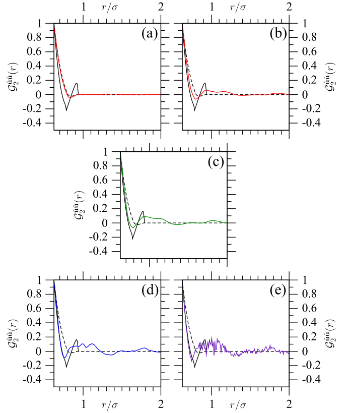
FIG. 6. Pair-correlation function G_2^{uu}(r) at several values of packing fraction \phi representative of the equilibrium fluid [(a) \phi = 0.378 ; (b) \phi = 0.614 ], metastable fluid [(c) \phi = 0.645 ], glassy [(d) \phi = 0.698 ], and MRJ [(e) \phi = 0.728 ] states. In each panel, the black curves correspond to the limit forms this function takes on when calculated considering two randomly chosen lenses either free (dashed) or touching (continuous).
