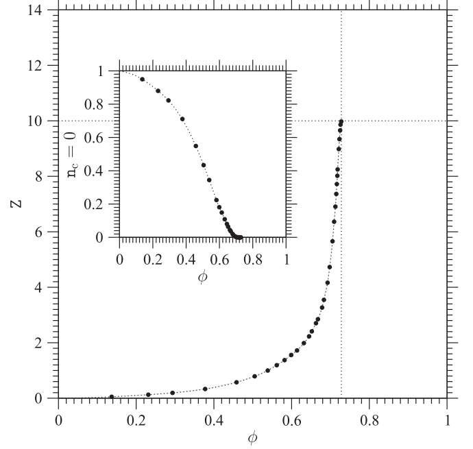
FIG. 10. Mean contact neighbor number Z as a function of packing fraction \phi (black circles and eye-guide dotted curve); the horizontal and vertical dotted lines intercept at (\phi_{\text{MRJ}}, 10) . The inset shows the number of “rattlers,” n_c = 0 , as a function of packing fraction \phi (black circles and eye-guide dotted curve).
