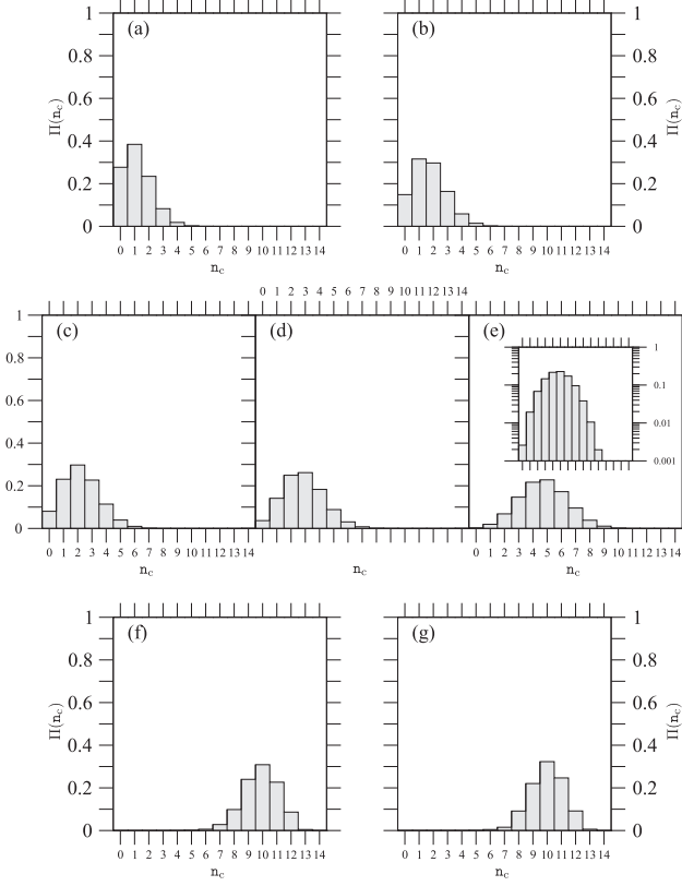
FIG. 9. Contact neighbor number probability \Pi(n_c) at several values of packing fraction \phi representative of the equilibrium fluid [(a) \phi = 0.562 ; (b) \phi = 0.614 ], metastable fluid [(c) \phi = 0.645 ], glassy [(d) \phi = 0.668 ; (e) \phi = 0.698 ], and (quasi)MRJ states [(f) \phi = 0.726 ; (g) \phi = 0.728 ]. In (e), the inset reproduces the main panel with the ordinate axis on a logarithm scale.
