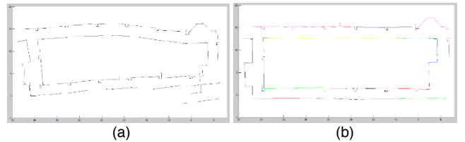
Figure 3: Illustration of region segmentation for plane-based modeling (a) Results with only one-time area mapping process. (b) Results with region segmentation and global alignment.
