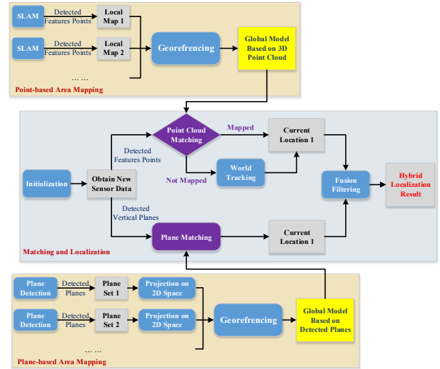
Figure 1: The proposed hybrid modeling and localization approach
