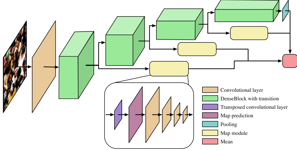
Figure 2: A diagram of the proposed network architecture MUD-ikNN: multiscale regression with DenseBlocks and ik NN mapping. Best viewed in color.
