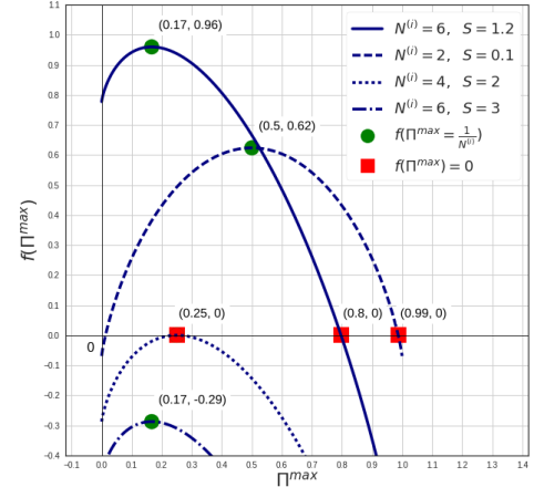
Fig. 2. Property of the maximum predictability. Three cases with and one case without solutions: N^{(i)} > 2^S , S \rightarrow 0 , N^{(i)} = 2^S , N^{(i)} < 2^S .
