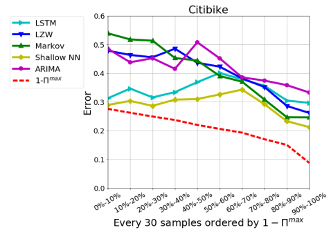
Supplementary Figure S9. Prediction errors of the Markov, LZW, NN, ARIMA and LSTM predictors using citibike data.
