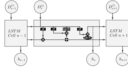
Supplementary Figure S4. LSTM predictor
