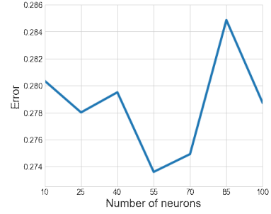
Supplementary Figure S3. sMAPE errors given the number of neurons per layer
