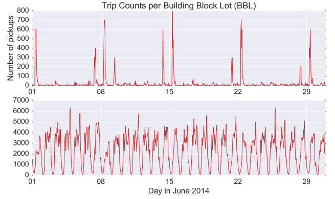
Fig. 1. Heterogeneous taxi demand time series in two building blocks: (top) a dense traffic area around the Metropolitan Museum of Art; and (bottom) a more open traffic area near the west port in NYC.
