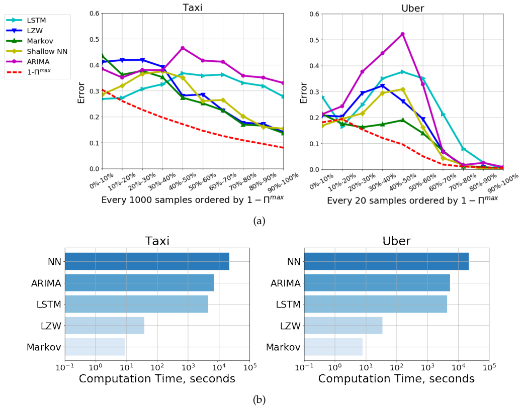
Fig. 6. (a) Prediction errors, (b) Computation time of the Markov, LZW, NN, ARIMA and LSTM predictors.
