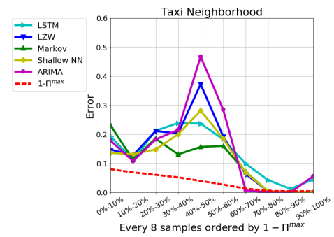
Supplementary Figure S7. Prediction errors of the Markov, LZW, NN, ARIMA and LSTM predictors at the neighborhood level.
