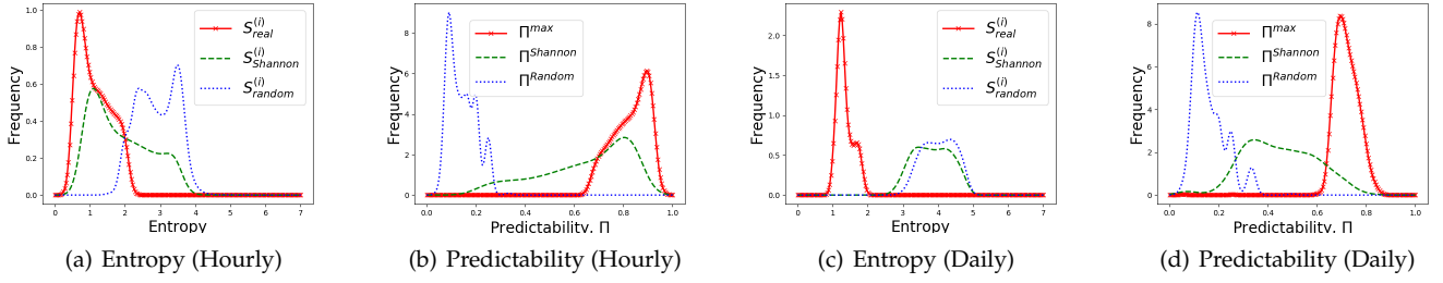
Fig. 3. Distribution of (a) Hourly Entropy, (b) Hourly Predictability, (c) Daily Entropy, and (d) Daily Predictability of the taxi demand over all building blocks. The red line, the green line and the blue line refer to the probability density function of S_{real}^{(i)} , S_{Shannon}^{(i)} , S_{random}^{(i)} and \Pi^{max} , \Pi^{Shannon} , \Pi^{random} in (a) (c) and (b) (d) respectively.
