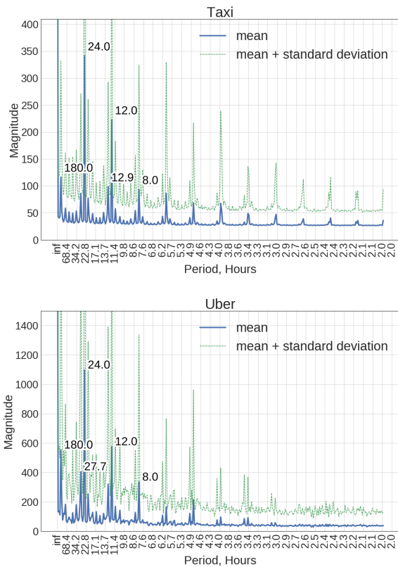
Supplementary Figure S5. Fourier transform with periods of the strongest magnitude for taxi and Uber data sets
