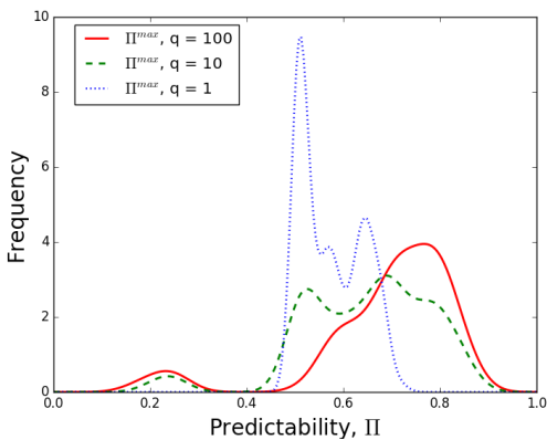
Supplementary Figure S6. Effect of of categorize size q
