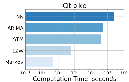
Supplementary Figure S10. Citi Bike prediction time
