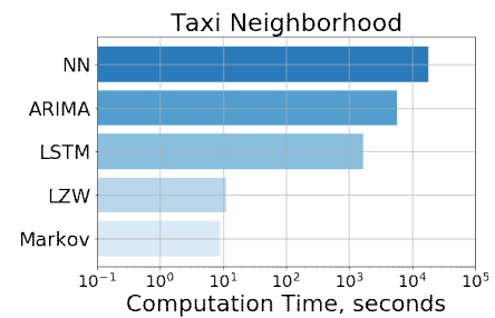
Supplementary Figure S8. Neighborhood prediction time.
