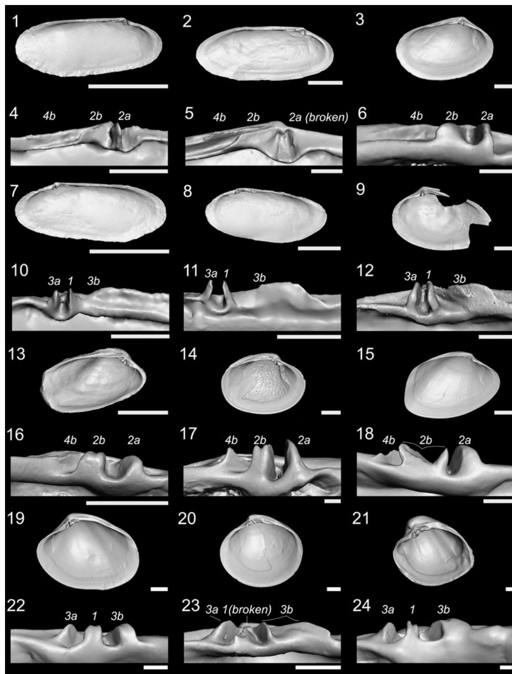
Figure 1. Exemplar specimens of Legumen and other Veneridae. Each specimen is illustrated as the whole valve with scalebar (10 mm) and an oblique close-up of the hingeplate (below, with a 2.5 mm scalebar) to facilitate comparison of dentition. Note that in Legumen ellipticum , unlike in the other modern and fossil Tapetinae illustrated here, teeth 1, 2b, and 3b are not bifid, and tooth 4b is extremely elongate. In Legumen carolinense , tooth 3b only is bifid, and the bifurcation is unlike that of true Tapetinae in orientation and character (see text). (1, 4) Legumen ellipticum Conrad, 1858 (USNM 76669, Nacatoch Formation, Kaufman County, Texas), left valve. (2, 5) Legumen ellipticum Conrad, 1858 (USNM 728210, Coon Creek Formation, Lee's Old Mill Site, Union County, Mississippi) left valve. (3, 6) Legumen carolinense (Conrad, 1875) (USNM 31947, "Black Creek Formation" (now Tar Heel Formation), Snow Hill, Greene County, North Carolina) left valve. (7, 10) Legumen ellipticum Conrad, 1858 (also USNM 76669) right valve (not included in the 3D analyses). (8, 11) Legumen ellipticum Conrad, 1858 (UFIP 180951, "Ripley Formation" (Owl Creek Formation), Owl Creek, Tippah County, Mississippi) right valve. (9, 12) Legumen carolinense (Conrad, 1875) (USNM 31802, "Black Creek Formation" (now Tar Heel Formation), Snow Hill, Greene County, North Carolina), right valve (not included in the 3D analyses). (13, 16) Irus irus (Linnaeus, 1758) (FMNH-IZ 176432, Recent, Monterey, California) left valve. (14, 17) Eurhomalea rufa (Lamarck, 1818) (FMNH-IZ 218326, Recent, Coquiambo, Chile) left valve. (15, 18) Tapes literatus (Linnaeus, 1758) (FMNH-IZ 293275, Recent, Broome, Western Australia) left valve. (19, 22) Ruditapes philippinarum (Adams and Reeve, 1850) (UF 173943, Recent, Pearl Harbor, Hawaii) right valve. (20, 23) Cyclorisma sp. (USNM 728211, "Black Creek Formation" (now Tar Heel Formation), Snow Hill, North Carolina) right valve; (21, 24) Eumaricia (Opimarcia) healyi (Marwick, 1948) (USNM 728212, Otahuhu Formation, Otahuhu Brewery Well, Auckland, NZ), right valve.
