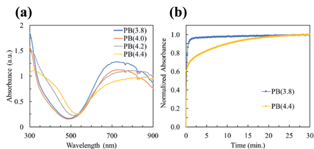
Fig. 4 UV-visible light absorbance spectra for FeHCF samples (a). Normalized optical absorbance at 700 nm during the first 30 minutes of synthesis (b).
