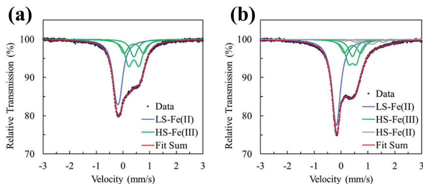
Fig. 6 Mössbauer spectra at room temperature of (a) PB(3.8) and (b) PB(4.4) with fitted Lorentzian curves representing iron species.
