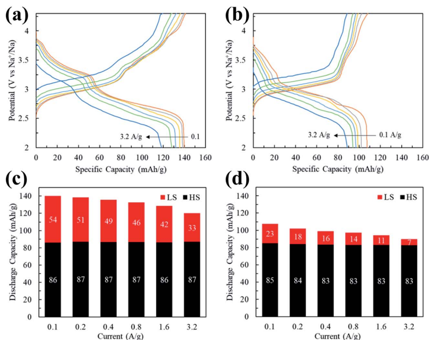
Fig. 11 Rate performance of PB(3.8) (a) and PB(4.4) (b), and their respective estimated capacity contributions between low-spin and high-spin Fe (c and d).
