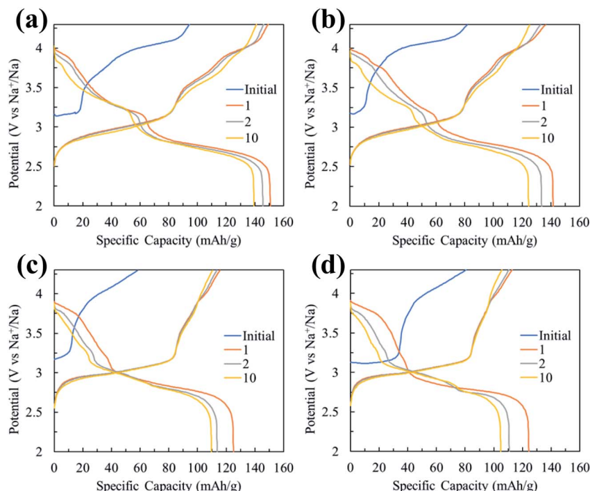
Fig. 8 Galvanostatic profile at 100 \text{ mA g}^{-1} of the initial charge and subsequent cycles for FeHCF synthesized with EDTA at pH 3.8 (a), pH 4.0 (b), pH 4.2 (c), and pH 4.4 (d).
