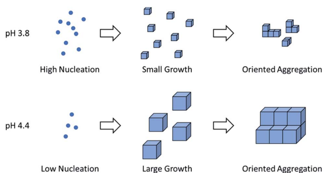
Fig. 3 Proposed mechanism of oriented aggregation between different synthesis pH.
