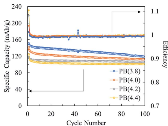
Fig. 9 Galvanostatic cycling at 100 \text{ mA g}^{-1} . Discharge shown as open circles and charge shown as filled circles.
