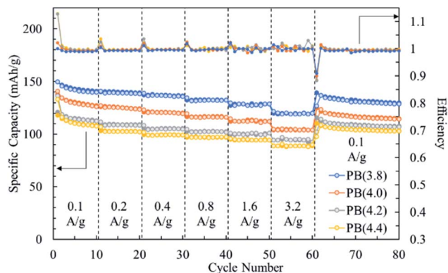
Fig. 10 Galvanostatic cycling at various current rates. Discharge shown as open circles and charge shown as filled circles.
