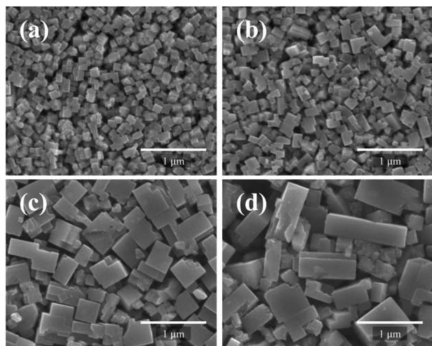
Fig. 2 SEM micrographs of (a) PB(3.8), (b) PB(4.0), (c) PB(4.2), and (d) PB(4.4). Scalebar is 1 \mu\text{m} .
