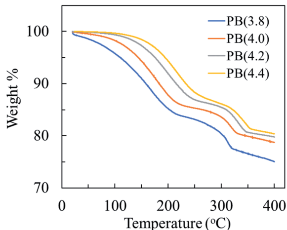
Fig. 5 TGA under nitrogen gas at 5\text{ }^{\circ}\text{C}^{-1}\text{ min} for FeHCF samples.
