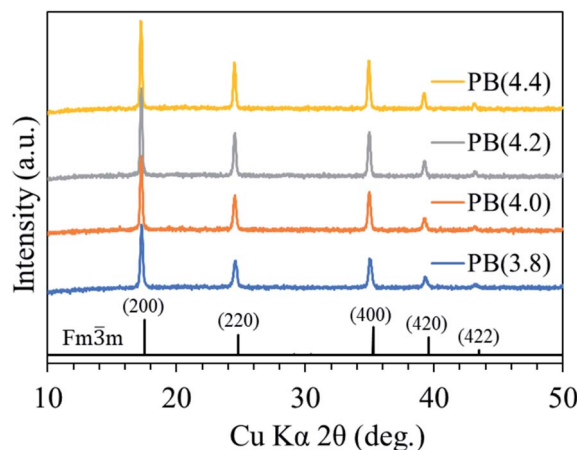
Fig. 1 XRD patterns of FeHCF samples between 10–50 degrees compared against ICDD no. 00-052-1907 for Prussian blue.
