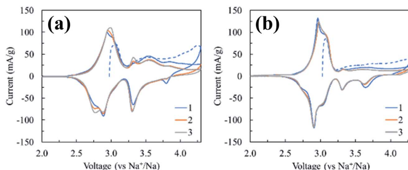
Fig. 7 Cyclic voltammetry at 0.1\text{ mV s}^{-1} for PB(3.8) (a) and PB(4.4) (b). Dashed line is initial charge.
