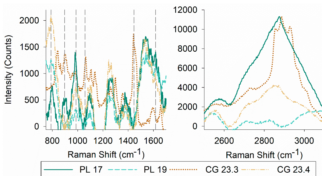
Figure 2. Raman spectra of biosurfactants: (left panel) wavenumbers from 750\text{--}1700\text{ cm}^{-1} and (right panel) from 2500\text{--}3100\text{ cm}^{-1} . Dashed lines indicate peaks at specific wavenumbers associated with biosurfactants.
