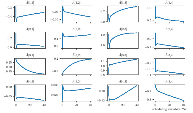
Fig. 4. The estimation of matrix functions as a function of p in the learned LPV-SS model (Take \hat{A} as an example). All the horizontal axes represent the scheduling variable PR . By approximating a smooth function for each matrix entry, the trained SIME model can predict the states and outputs of a system with high accuracy.
