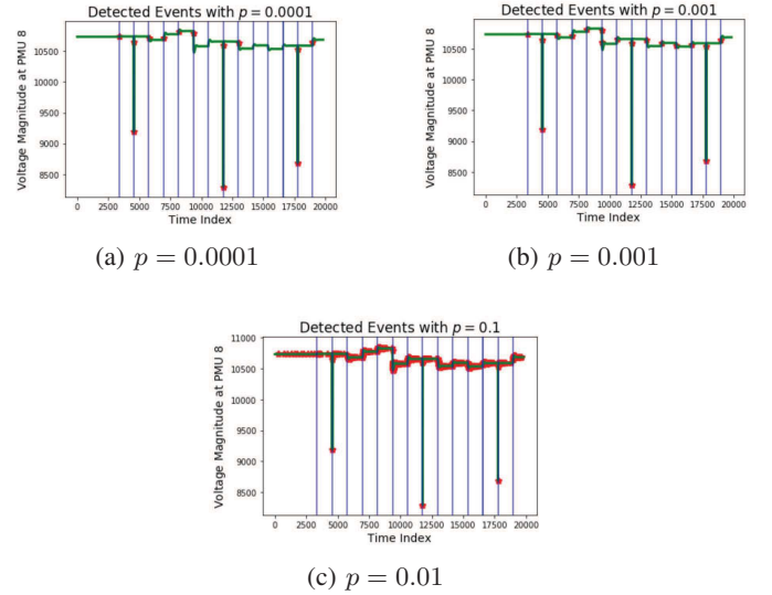
Fig. 2: (a)-(c) Visualization of event detection performance on one stream of PMU measurements for different choices of anomaly threshold probability ( p ). Vertical blue lines indicate ground truth of event occurrence. Red stars indicate events flagged by algorithm.
