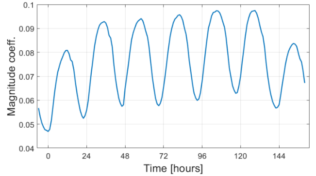
Fig. 2. Temporal profile corresponding to the largest singular value. Each hour multiple of 24 indicates midnight of the corresponding day.
