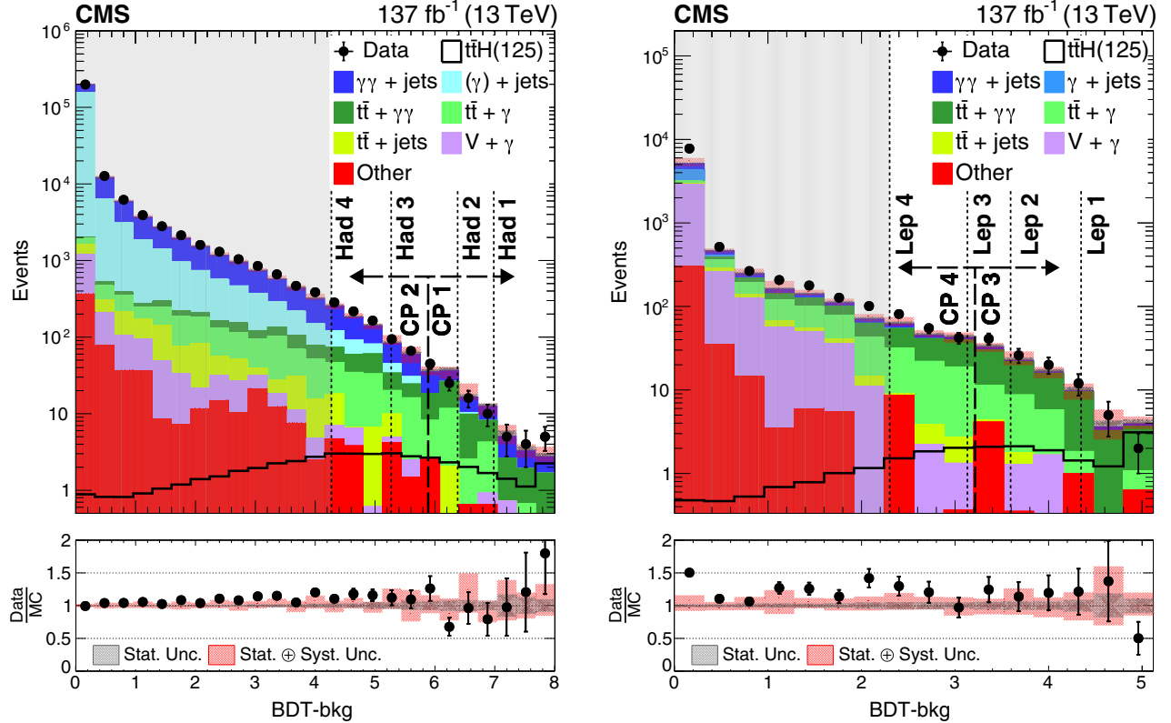
FIG. 1. Distributions of BDT-bkg output used for event categorization for the hadronic (left) and the leptonic (right) channels. Category boundaries for the signal strength ( CP ) measurements are shown with thinly (thickly) dashed lines. Events shown are taken from the m_{\gamma\gamma} sidebands, satisfying either 100 < m_{\gamma\gamma} < 120 GeV or 130 < m_{\gamma\gamma} < 180 GeV. Events in the gray shaded region are not considered in the analysis. Statistical (statistical \oplus systematic) background uncertainties are represented by the black (red) shaded bands.
