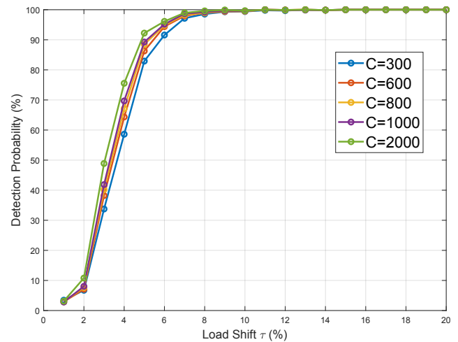
Fig. 5: Effect of outlier penalty factor C on testing random attack detection probability. Data is shown for \tau_{\min} = 3\% .
