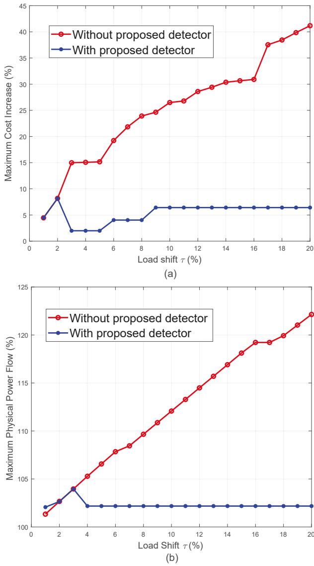
Fig. 7: Mitigation results of (a) CM attacks and (b) LO attacks. For each load shift, the points on the red lines indicate the worst consequence as a result of attack, and the points on the blue lines indicate the worst consequence with our attack detection framework. Points on the blue line are obtained by taking the maximum of two quantities: (i) resulting worst consequence if re-dispatch using SVR predicted loads when attack is flagged; and (ii) the worst attack consequence when the detector fails.
