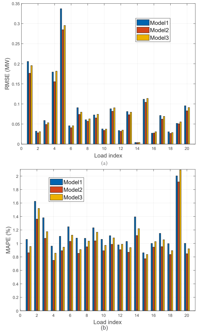
Fig. 2: Performance of the SVR models under two metrics: (a) RMSE, and (b) MAPE. Model 1 does not capture spatial correlations. Model 2 uses temporal features of 3 previous hours and 2 previous days. Model 3 uses temporal features of 4 previous hours and 3 previous days. Both Models 2 and 3 capture spatial correlation.
