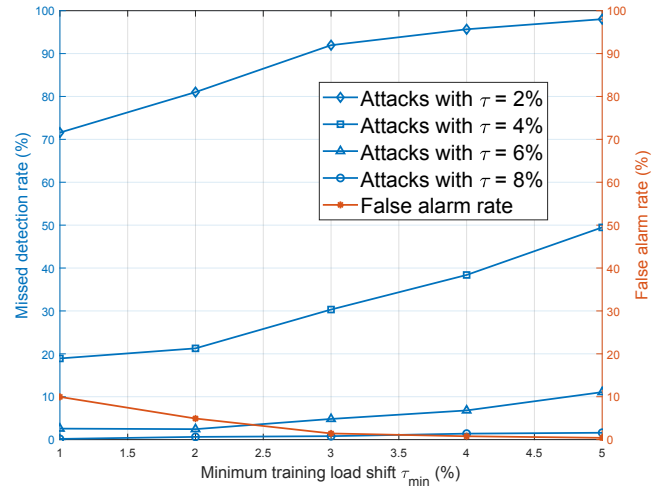
Fig. 4: Effect of minimum training load shift \tau_{\min} . False alarm rate and missed detection rate when testing random attacks are each plotted as a function of \tau_{\min} . Data is shown for C = 1000 .
