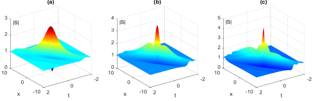
FIG. 6: Bright RWs with single main hump for SW in the LWSW model (1)-(2) given by the parameters \rho = \sigma = a_0^{(0)} = 1 , a_2^{(0)} = a_4^{(0)} = 0 , \alpha = 3 : (a) first-order case; (b) second-order case; (c) third-order case.
