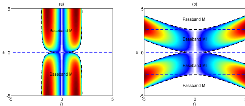
FIG. 7: MI for the LWSW model (1)-(2) on the (\Omega, \omega) plane calculated with the parameters a = 1 , b = 0 , and (a) \sigma = 1 ; (b) \sigma = -1 . Dark dashed curves indicate the analytical marginal stability condition \Delta = 0 .
