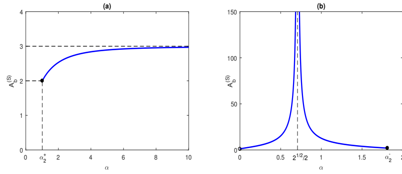
FIG. 3: The maximum amplitude of the bright RW for SW in the LWSW model (1)-(2) with the parameters \rho = 1 and (a) \sigma = 1 ; (b) \sigma = -1 .
