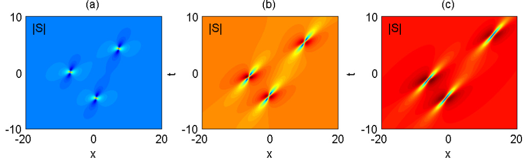
FIG. 4: Second-order RW for SW in the LWSW model (1)-(2) with the parameters \rho = -\sigma = 1 , a_0^{(0)} = 1 , a_1^{(0)} = a_2^{(0)} = 0 , a_3^{(0)} = 350 and (a) bright state \alpha = 1.5 ; (b) intermediate state \alpha = 2.1 and (c) dark state \alpha = 2.3 .
