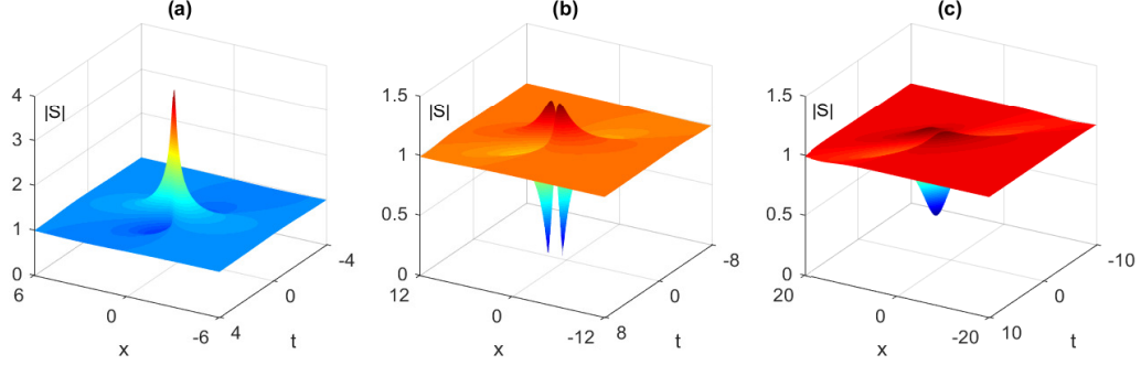
FIG. 1: First-order RW for SW in the LWSW model (1)-(2) with the parameters \rho = -\sigma = 1 and (a) bright state \alpha = 1.5 ; (b) intermediate state \alpha = 2.1 and (c) dark state \alpha = 2.3 .
