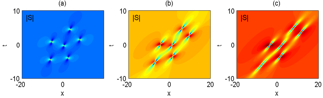
FIG. 5: Third-order RW for SW in the LWSW model (1)-(2) with the parameters \rho = -\sigma = 1 , a_0^{(0)} = 1 , a_1^{(0)} = a_2^{(0)} = a_3^{(0)} = a_4^{(0)} = 0 , a_5^{(0)} = 2000 and (a) bright state \alpha = 1.5 ; (b) intermediate state \alpha = 2.1 and (c) dark state \alpha = 2.3 .
