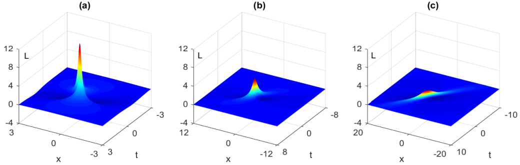
FIG. 2: First-order RW for LW in the LWSW model (1)-(2) with the parameters \rho = -\sigma = 1 and (a) \alpha = 1.5 ; (b) \alpha = 2.1 and (c) \alpha = 2.3 , respectively.
