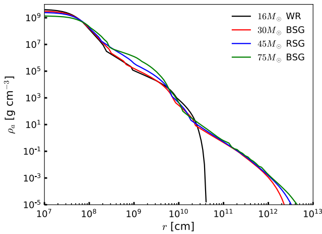
FIG. 1. Left panel: Progenitor density profiles from [47]. Right panel: Jet head location r_h and collimation shock radius r_{\text{cs}} as a function of time. The solid lines correspond to the points obtained from Eq. (1) and Eq. (2), while the dashed lines are the associated extrapolations.
