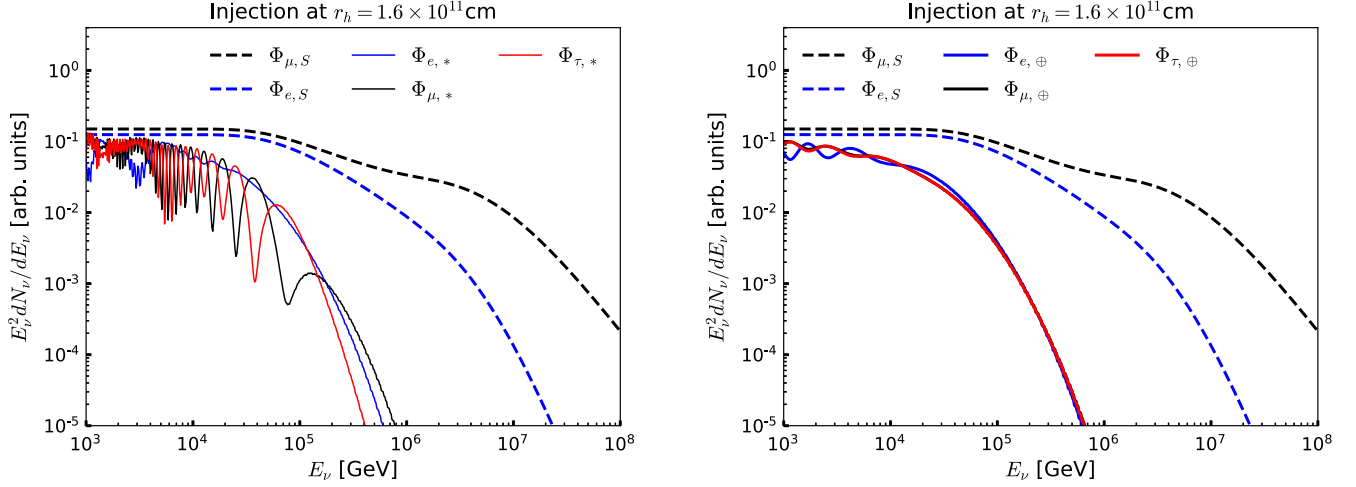
FIG. 2. Neutrino energy spectrum from a choked LP GRB jet inside a BSG. Left panel: Neutrino spectrum after propagating from the injection site, r_h = 1.6 \times 10^{11} cm, to edge of the source. Right panel: Same as left panel, showing the flux arriving at Earth after averaging out due to long distance propagation. The proton flux is normalized such that E_p^2 dN_p/dE_p = 1 . The \nu_\alpha + \bar{\nu}_\alpha spectra at injection are represented by the dashed curves, combining contributions from \pi and \mu decay after accounting for cooling.
