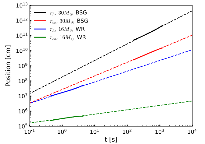
FIG. 1. Left panel: Progenitor density profiles from [47]. Right panel: Jet head location r_h and collimation shock radius r_{\text{cs}} as a function of time. The solid lines correspond to the points obtained from Eq. (1) and Eq. (2), while the dashed lines are the associated extrapolations.
