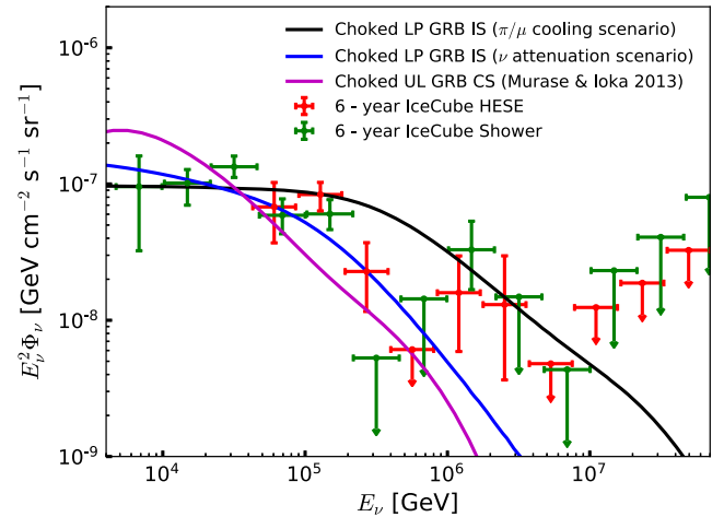
FIG. 6. All flavor choked LP GRB diffuse neutrino fluxes in comparison with the IceCube astrophysical neutrino spectra. The data from the 6-year shower analysis [62] is shown by the green bars, while the result of the 6-year HESE analysis [63] is shown by the red bars. The per-flavor neutrino flux from [63] was multiplied by a factor of 3 to estimate the all-flavor flux. The \pi/\mu cooling scenario uses L_{\text{iso},48} = 2 , \Gamma_j = 70 , \theta_j = 0.2 , t_{\text{dur}} = 2000 s, and a 75 M_{\odot} BSG progenitor, while the \nu attenuation scenario assumes L_{\text{iso},48} = 1 , \Gamma_j = 50 , \theta_j = 1 , t_{\text{dur}} = 1800 s, and a 30 M_{\odot} BSG progenitor. The remaining parameters are given in Table I. For comparison, we show the spectrum of the choked UL GRB neutrinos from the collimation shock (CS) in Ref. [11] but the flux is rescaled.
