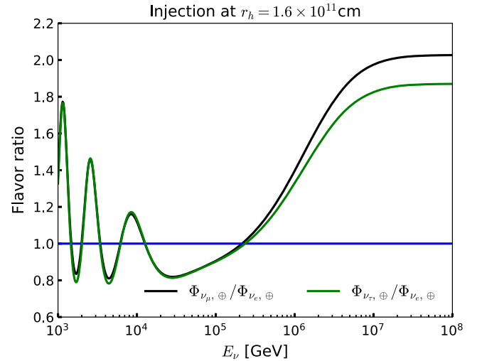
FIG. 3. Observed \Phi_{\nu_\alpha}/\Phi_{\nu_e} flavor ratios on the Earth (i.e., oscillations are averaged out). Neutrino spectra are injected at r_h = 1.6 \times 10^{11} cm. The blue line is a line for the (1 : 1) ratio and is added as a reference.
