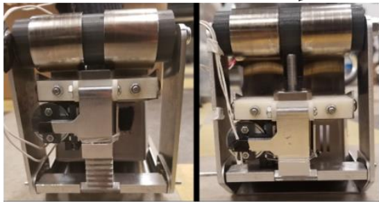
b) LOCKING MECHANISM DESIGN UNLOCKED (LEFT) V.S. LOCKED (RIGHT)
