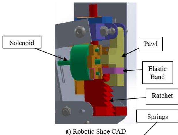
a) Robotic Shoe CAD
