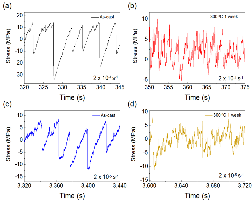
Figure 3. Graphs for the detrended stress vs. time curves for the (a) as-cast \text{Zr}_{52.5}\text{Cu}_{17.9}\text{Ni}_{14.6}\text{Al}_{10}\text{Ti}_5 BMG compressed at a strain rate of 2 \times 10^{-4} \text{ s}^{-1} , (b) thermally-annealed (300 °C, 1 week) \text{Zr}_{52.5}\text{Cu}_{17.9}\text{Ni}_{14.6}\text{Al}_{10}\text{Ti}_5 BMG compressed at a strain rate of 2 \times 10^{-4} \text{ s}^{-1} , (c) as-cast \text{Zr}_{52.5}\text{Cu}_{17.9}\text{Ni}_{14.6}\text{Al}_{10}\text{Ti}_5 BMG compressed at a strain rate of 2 \times 10^{-5} \text{ s}^{-1} , and (d) thermally-annealed (300 °C, 1 week) \text{Zr}_{52.5}\text{Cu}_{17.9}\text{Ni}_{14.6}\text{Al}_{10}\text{Ti}_5 BMG compressed at a strain rate of 2 \times 10^{-5} \text{ s}^{-1} .
