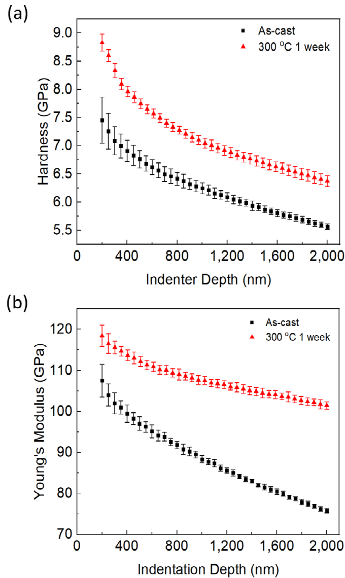
Figure 2. (a) Nanoindentation hardness vs. indentation depth for the as-cast and annealed (300 °C, 1 week) \text{Zr}_{52.5}\text{Cu}_{17.9}\text{Ni}_{14.6}\text{Al}_{10}\text{Ti}_5 BMG samples. (b) Nanoindentation Young's modulus vs. indentation depth for the as-cast and annealed (300 °C, 1 week) \text{Zr}_{52.5}\text{Cu}_{17.9}\text{Ni}_{14.6}\text{Al}_{10}\text{Ti}_5 BMG samples for indentations depths ranging from 200 to 2000 nm.
