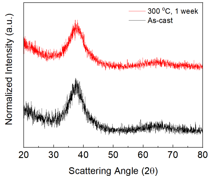
Figure 1. The XRD patterns for the as-cast and annealed Zr_{52.5}Cu_{17.9}Ni_{14.6}Al_{10}Ti_5 bulk metallic glass (BMG) samples.
