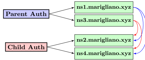
Fig. 2: Disjoint NSSet Experiment for marigliano.xyz
