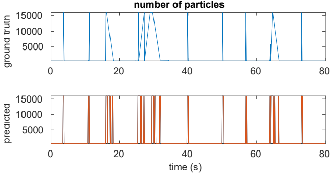
Figure 6: Ground truth and predicted number of particles using RUSBoost on AMCL running on Intel i5-3317u.
