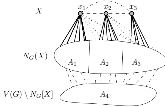
■ Figure 4 The partition on V(G) in the proof of Lemma 6. Solid and dotted lines respectively indicate that a vertex is complete or anti-complete to a set. Dashed edges might, but do not have to exist.
