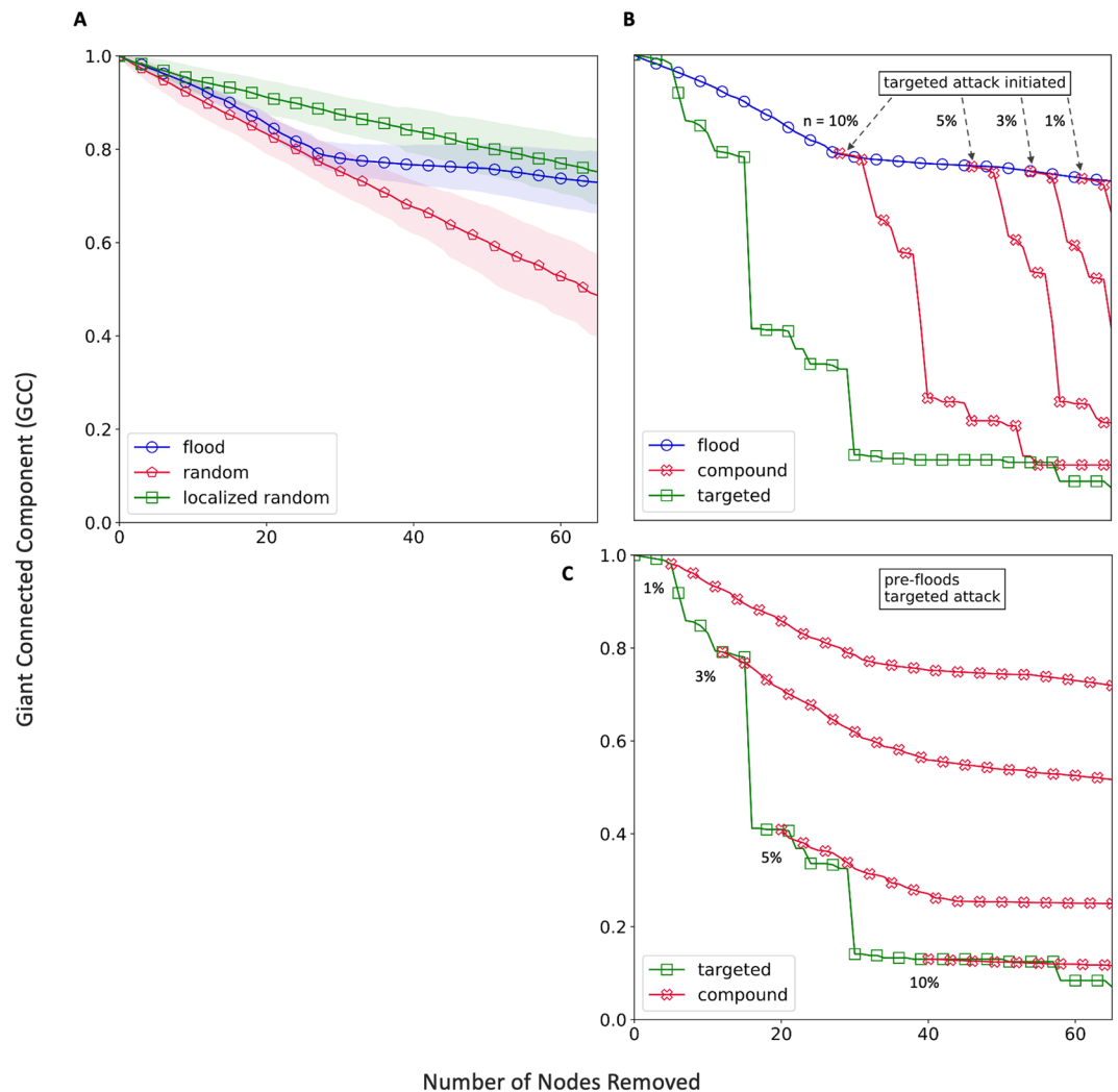
Figure 3. Robustness of the London Rail network under (A) flood failure and two types of random failure (overall and localized). (B) compound failure where n\% nodes (of total) are removed in a targeted manner after certain nodes have failed due to flooding. (C) compound failure with targeted attack before flooding.
