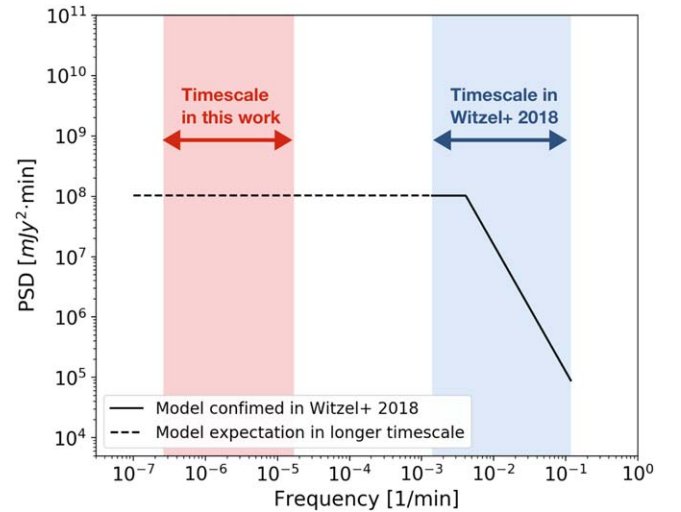
Figure 10. Modeled PSD of Sgr A* presented in Witzel et al. (2018). The solid line shows the broken power-law PSD that has been confirmed in previous short-term variability observations with a break timescale of \tau \sim 245 minutes. The dashed line shows the assumed flat PSD in a longer timescale. The blue band marks the timescale probed in existed studies, and the red band marks the timescale that we explored in this work.
