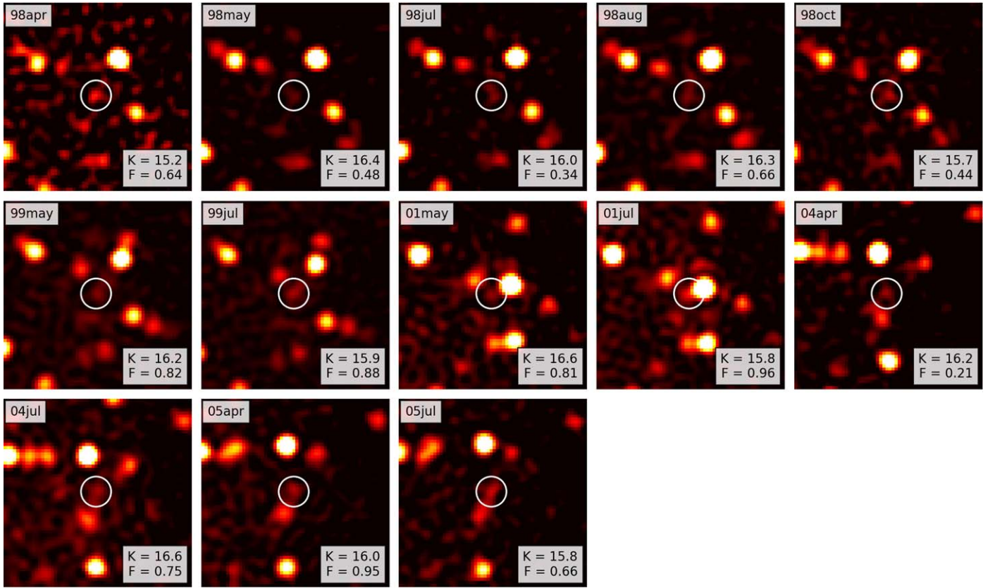
Figure 5. Speckle holography images with new Sgr A* detections (white circles). For each detection, the K magnitude ( K ) and the bootstrap fraction ( F ) are provided. These are the first IR detections of Sgr A* in the late 1990s and early 2000s.
