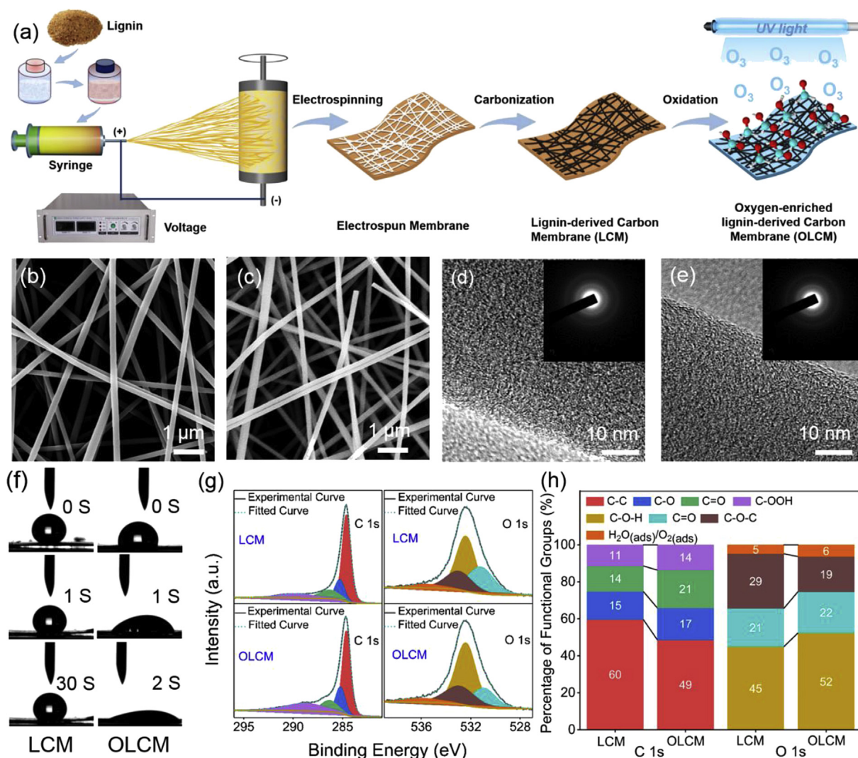
Fig. 1. (a) Schematic diagram of the fabrication process of the LCM and OLCM. (b, c) Representative SEM images of the LCM and OLCM, respectively. (d, e) TEM images of LCM and OLCM, respectively. Insets: selected area electron diffraction (SAED). (f) Water contact angle images of the LCM and OLCM. (g) XPS C 1s and O 1s spectra of the LCM and OLCM. (h) Quantification of the functional groups present on the surfaces of LCM and OLCM. The same color codes apply to (g) and (h). (For interpretation of the references to color in this figure legend, the reader is referred to the Web version of this article.)
