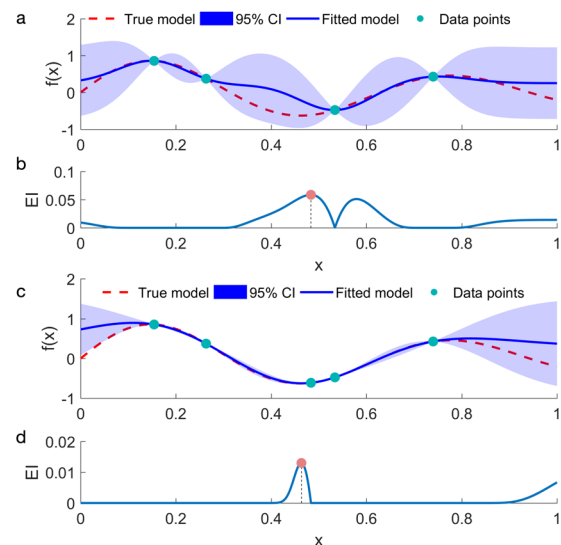
Figure 9. GP model evolution using EI as the acquisition function: (a) initial GP model based on four data points, (b) EI of the initial GP model, (c) updated GP model after sampling one additional data point based on EI, (d) EI of the updated GP model.
