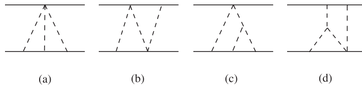
FIG. 14. (a) Three-graviton emission from one of the bodies; (b) symmetric three-graviton exchange; (c) composition of a three-graviton vertex with a two-graviton vertex in the source term.
