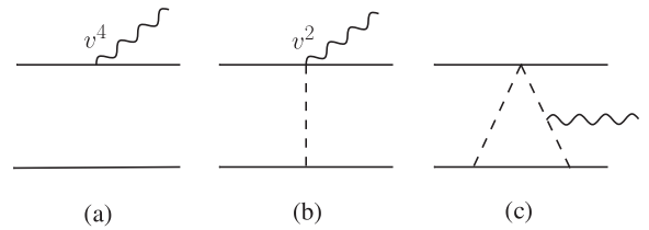
FIG. 7. Diagrams with \bar{h}^{ii} external momentum.
