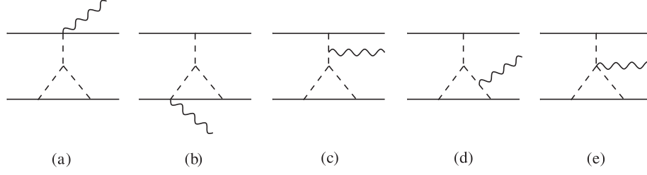
FIG. 5. Three-potential-graviton exchange with external \bar{h}^{00} momentum.
