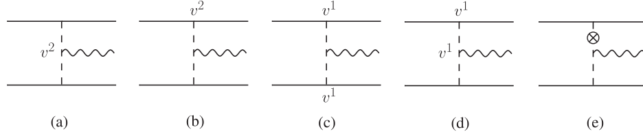
FIG. 8. One potential graviton exchange with \bar{h}^{ii} external momentum.
