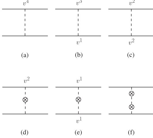
FIG. 12. Diagrams with one-graviton exchange.
