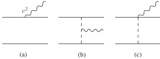
FIG. 10. Diagrams (a) and (b) contribute to T_{\text{0PN}}^{ij} when the external leg is \bar{h}^{ij}(x) , while diagrams (a), (b), and (c) contribute to T_{\text{1PN}}^{00} when we consider \bar{h}^{00}(x) as the external leg.
