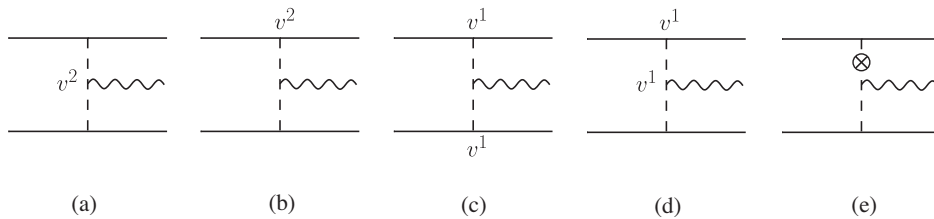
FIG. 3. Diagrams with two potential gravitons coupled to \bar{h}_{00} .
