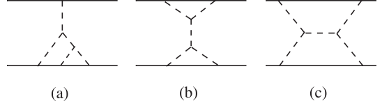
FIG. 17. Diagrams with five propagators.
