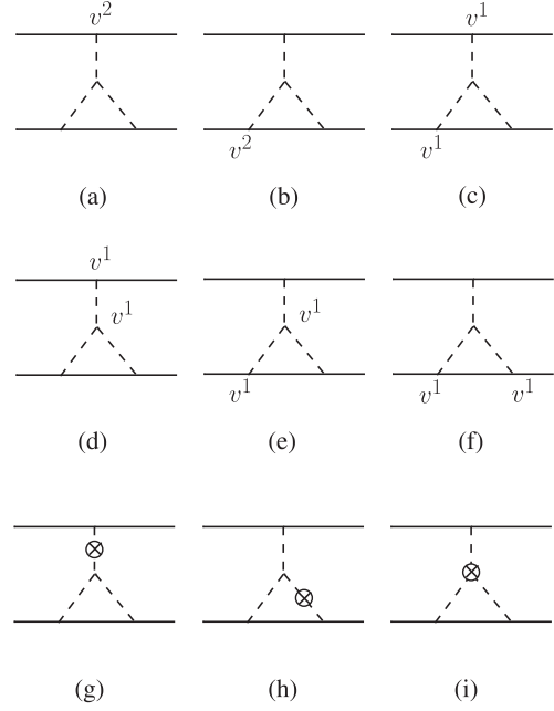
FIG. 15. Diagrams with three-graviton exchange.
