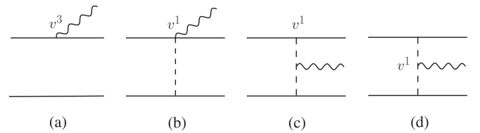
FIG. 6. All diagrams that contribute to T_{1\text{PN}}^{0i} .
