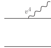
FIG. 1. No graviton exchange between the two particles, one external \bar{h}^{00} momentum.
