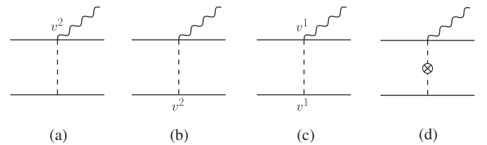
FIG. 2. One-graviton exchange with external \bar{h}^{00} momentum.
