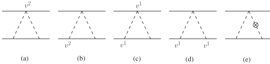
FIG. 13. Diagrams with two-graviton exchange.
