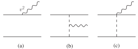
FIG. 9. Three-potential-graviton exchange with \bar{h}^{ii} external momentum.
