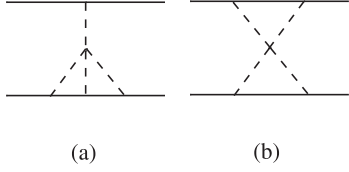
FIG. 16. Diagrams with four-graviton vertex.
