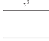
FIG. 11. Diagram with no graviton exchange.
