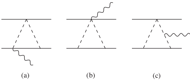
FIG. 4. Two-potential-graviton exchange with external \bar{h}^{00} momentum.
