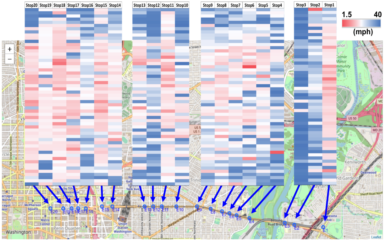
Figure 8: Average speed of each (bus stop, time) pair.
