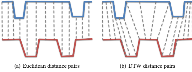
Figure 5: Example of the Euclidean vs. the DTW distance between two bus stop speed signatures, shown in blue and in red color respectively, with two slowdowns each. Each dashed line indicates the matching between a point in the first time series and its match in the second time series.
