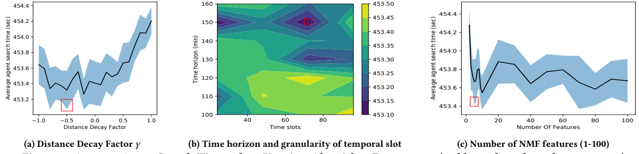
(a) Distance Decay Factor \gamma (b) Time horizon and granularity of temporal slot (c) Number of NMF features (1-100) Figure 3: Average Agent Search Time when Varying Algorithm Parameters (red box: the selected parameters)
