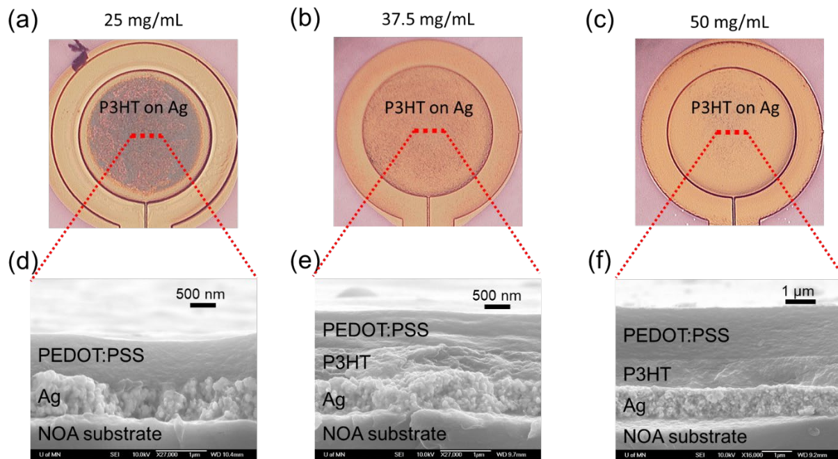
Figure 4. (a-c) top view optical images of annealed P3HT films deposited using inks with a P3HT concentration of (a) 25 mg/mL, (b) 37.5 mg/mL and (c) 50 mg/mL. (d-f) cross-sectional SEM images for completed devices taken along the red dashed lines shown in (a-c)
