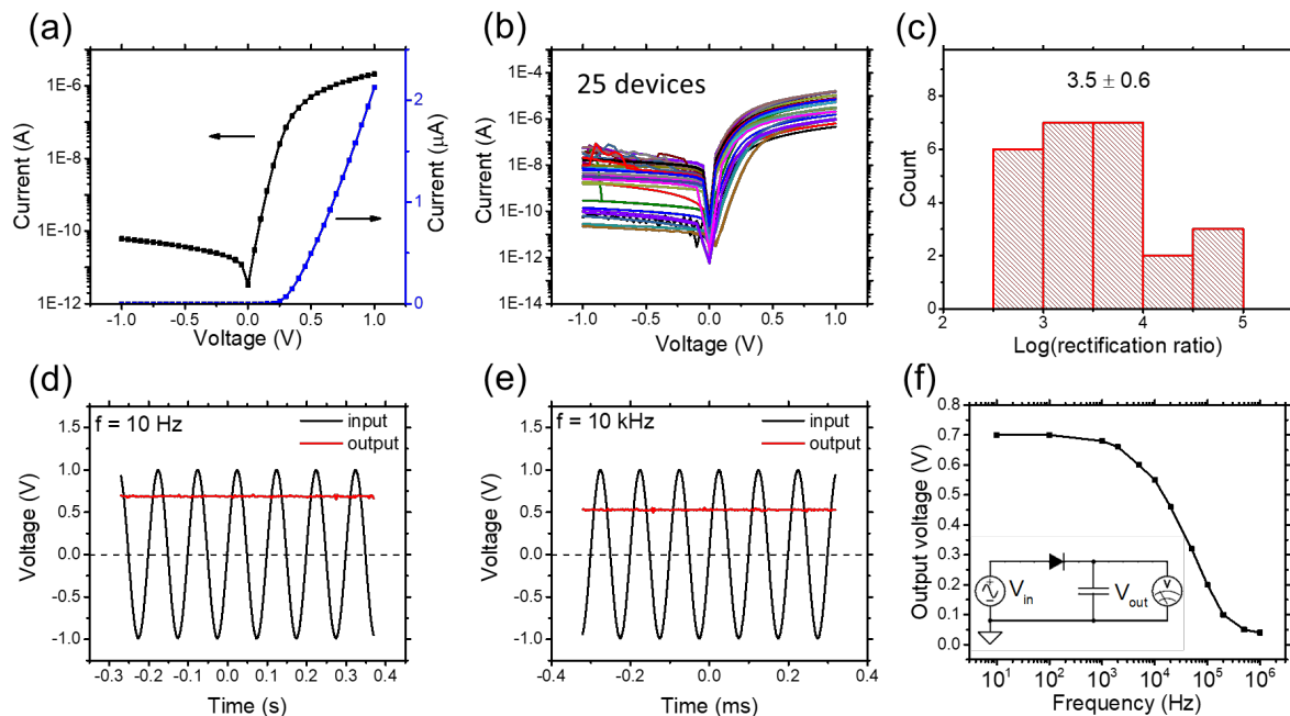
Figure 5. Static and dynamic electrical performances of printed diodes (a) IV characteristic of a printed diode. (b) IV curves collected from 25 printed diodes and (c) histogram of log(rectification ratio) of these devices. (d-) dynamic performance of a rectifier circuit (shown in the inset image in (f)) at an input frequency of (d) 10 Hz and (e) 10 kHz. (f) Output voltage as a function of input frequency for the rectifier circuit in the inset image. The capacitor connected in series with the diode is 1 \mu F.
