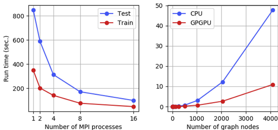
Fig. 2. (a) Scaling of iScore.train.mpi and iScore.predict.mpi with respect to the number of MPI processes. The training and testing set contained 234 and 599 conformations respectively. (b) Average run time on CPU (Intel Xeon E5-2650 v4 @ 2.20 GHz) and GPU (Nvidia GeForce GTX 1080 Ti) for the calculation of RWGK for two graphs containing n nodes and 3n edges.
