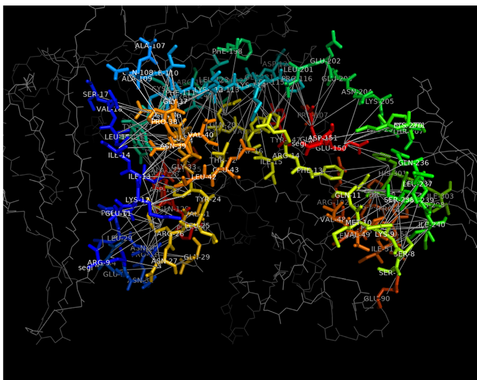
Fig. 3. Visualization of the connection graph of PDB ID: 1IRA using iScore.h5x with the PyMol molecular viewer. All interface residues are colored differently following a rainbow color palette to facilitate their identification. The residues that are not part of the interface are represented as thin gray lines. The connection between interface residues are shown as white lines. (For interpretation of the references to color in this figure legend, the reader is referred to the web version of this article.)
