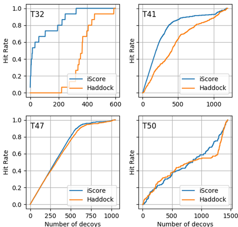
Fig. 4. Comparison of the hit rates obtained by iScore and HADDOCK for four CAPRI targets.
