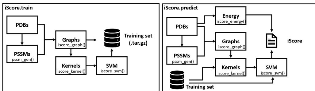
Fig. 1. Computational workflow of iScore during the training of a SVM model and during the utilization of pre-trained model to rank new PPIs.
