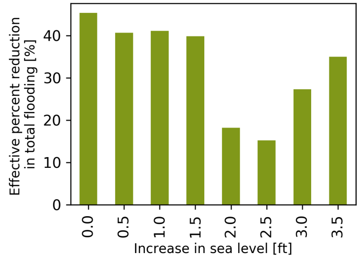
Figure 7: Effective percent total flood reduction in MPC compared to tide gate scenario given increasing sea level
