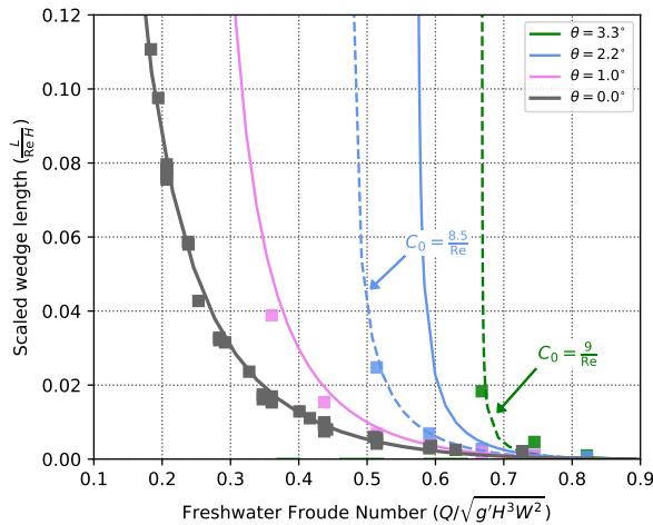
FIGURE 9. Equilibrium wedge length as in figure 6b, but including results from the sloped channel experiments. Squares indicate experimental data while solid lines represent theoretical predictions, assuming \hat{C}_i = \hat{C}_d and C_0 = 7/\text{Re} . The line for \theta = 3.3^\circ is not shown since the theory predicts infinite salt-water intrusions for the chosen range of \text{Fr}_0 . Dashed lines are like the solid lines but with C_0 = 8.5/\text{Re} and C_0 = 9/\text{Re} for the \theta = 2.2^\circ and \theta = 3.3^\circ cases, respectively.
