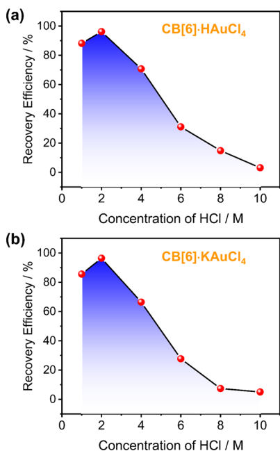
Figure 4. Effect of changes in the concentration of HCl on gold-recovery efficiency from two coprecipitated adducts (a) \text{CB}[6] \cdot \text{HAuCl}_4 and (b) \text{CB}[6] \cdot \text{KAuCl}_4 . The concentrations of \text{CB}[6] and \text{MAuCl}_4 in all aqueous solutions are 6 mM.
