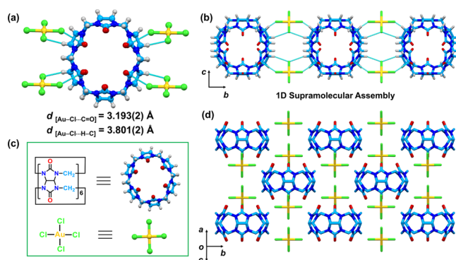
Figure 5. Solid-state superstructure of the adduct formed between \text{CB}[6] and \text{H[AuCl}_4] . (a) Ball-and-stick representation showing that every \text{CB}[6] molecule interacts with four [\text{AuCl}_4]^- anions through [\text{Au}-\text{Cl} \cdots \text{H}-\text{C}] hydrogen-bonding and ion-dipole interactions. (b) Supramolecular assembly of the one-dimensional nanostructure extending along the b axis in which adjacent \text{CB}[6] molecules are connected by two parallel aligned [\text{AuCl}_4]^- anions. (c) Structural formulas of \text{CB}[6] and [\text{AuCl}_4]^- anions. (d) Solid-state superstructure of \text{CB}[6] \cdot \text{HAuCl}_4 , which is made up of the parallel aligned 1D supramolecular assemblies illustrated in (b). The \text{H}_2\text{O} molecules are omitted for the sake of clarity. H: gray, C: pale blue, N: blue, O: red, Cl: green, and Au: yellow.
