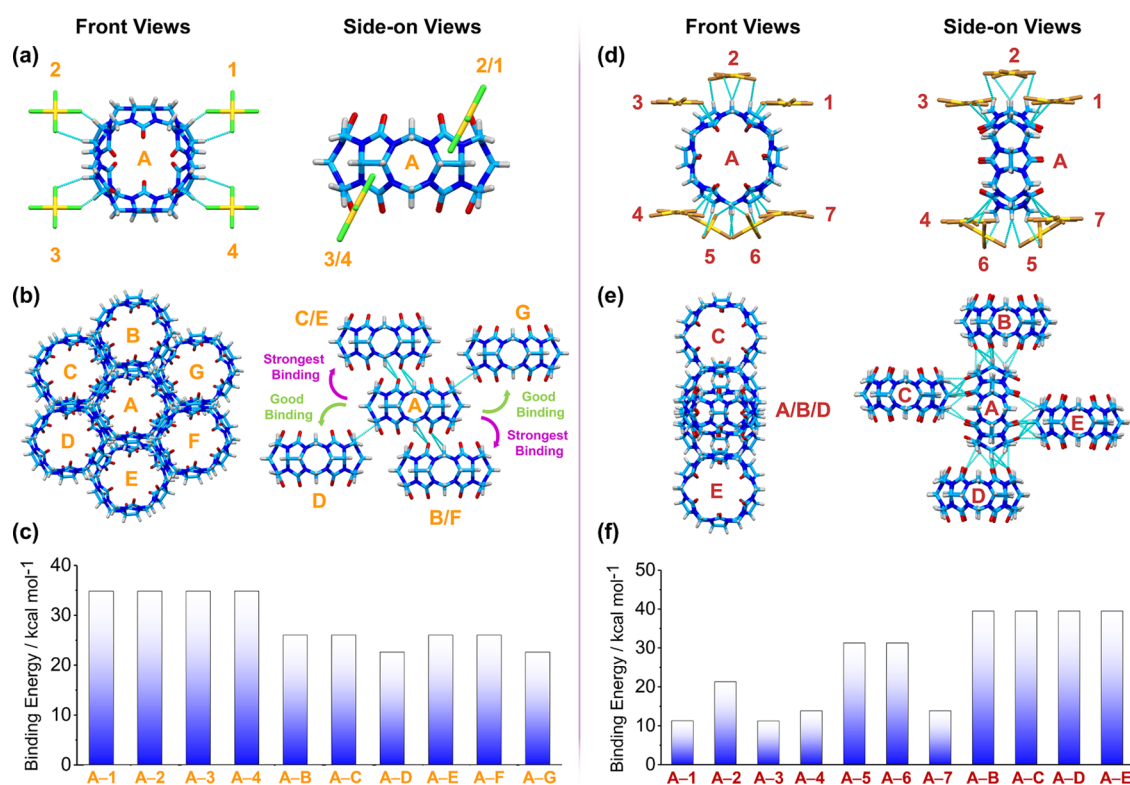
Figure 7. Solid-state superstructures and binding energies between CB[6] and [AuX 4 ] − (X = Cl/Br) anions obtained by DFT calculations. (a, b) Capped-stick representation illustrating the different views of how CB[6] (A) interacts with four [AuCl 4 ] − anions (1–4) and six adjacent CB[6] molecules (B–G) in the solid-state superstructures of CB[6]·HAuCl 4 . (c) Results of DFT calculations of the binding energies between CB[6] (A) and four connected [AuCl 4 ] − anions (1–4) in addition to six adjacent CB[6] molecules (B–G). (d, e) Capped-stick representation illustrating different views of how CB[6] (A) interacts with seven [AuBr 4 ] − anion (1–7) and four adjacent CB[6] molecules (B–E) in the solid-state superstructures of CB[6]·HAuBr 4 . (f) Results of DFT calculations on the binding energies between CB[6] (A) and seven connected [AuBr 4 ] − anions in addition to four adjacent CB[6] molecules (B–E). A–X (X = 1–7/B–G) representing the two interacting molecules defined in Figure 7. H: gray, C: pale blue, N: blue, O: red, Cl: green, Br: brown, and Au: yellow.
