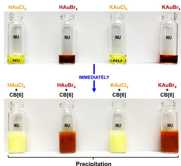
Figure 1. Formation of coprecipitates of \text{CB}[6] \cdot \text{MAuX}_4 ( M = \text{H}/\text{K} , X = \text{Cl}/\text{Br} ) from CB[6] and \text{MAuX}_4 . When CB[6] (8 mM, 1.5 mL) in an aqueous HCl (3 M) or HBr (3.5 M) solution is added to aqueous solutions of \text{MAuX}_4 (20 mM, 0.6 mL), yellow or brown coprecipitates, respectively, are formed immediately. See Supplementary Movie 1.
