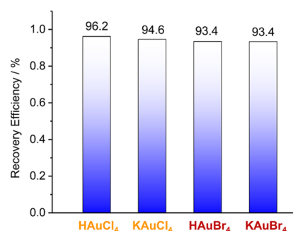
Figure 2. Gold-recovery efficiencies based on the coprecipitates from four aqueous solutions of CB[6] (5.7 mM) and \text{MAuX}_4 (5.7 mM) ( M = \text{H}/\text{K} , X = \text{Cl}/\text{Br} ), calculated according to the initial and residual concentrations of [\text{AuX}_4]^- anions in the aqueous solutions which were measured at 25^\circ \text{C} by ICP-OES analysis.
