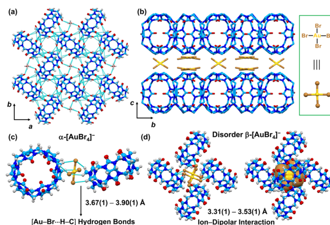
Figure 6. Solid-state superstructure of the adduct formed between CB[6] and H[AuBr 4 ]. (a) Supramolecular assembly of the 2D nanostructure in the a – b plane as a result of multiple hydrogen bonds between H 2 O and CB[6] molecules, as well as between two adjacent CB[6] molecules. (b) Solid-state superstructure of CB[6]·HAuBr 4 in which two polymorphs of the [AuBr 4 ] − — \alpha -[AuBr 4 ] − and \beta -[AuBr 4 ] − —anion are accommodated in the lattice between the 2D supramolecular assemblies illustrated in (a). (c) Ball-and-stick representation showing that every \alpha -[AuBr 4 ] − anion interacts with two CB[6] molecules through [Au–Br···H–C] hydrogen bonds. (d) \beta -[AuBr 4 ] − anions interact with five CB[6] molecules, which are disordered over two positions with 50:50 occupancies. H: gray, C: pale blue, N: blue, O: red, Br: brown, and Au: yellow.
