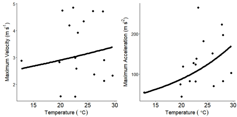
Figure 1: Scatterplots of maximum strike velocity and maximum strike acceleration for Mojave rattlesnakes in the field experiment. Regression lines are back-transformed predictions from the mixed models. Temperature had a statistically significant effect on maximum acceleration, but not maximum velocity.
